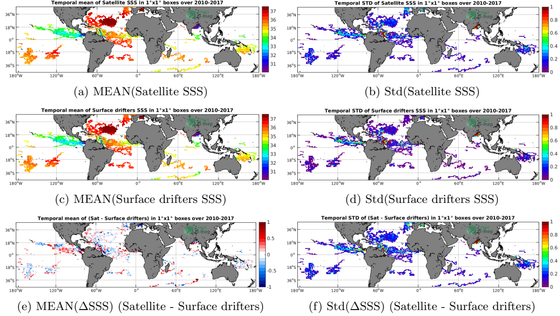
Figure 5: Temporal mean (left) and Std (right) of SSS from SMOS-L3-CATDS-CECOS-LOCEAN-V4-9DAYS-25KM (top), Surface drifters (middle), and of \Delta SSS (Satellite - Surface drifters). Only match-up pairs are used to generate these maps.
