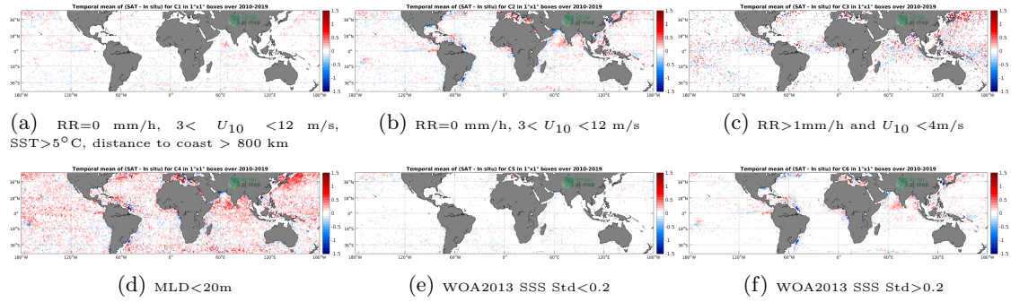
Figure 12: Temporal mean gridded over spatial boxes of size 1^\circ \times 1^\circ of \Delta SSS (SMOS SSS L3 v4 - 9 Days (CATDS-CECOS-LOCEAN) - Argo) for 6 different subdatasets corresponding to: RR=0 mm/h, 3 < U_{10} < 12 m/s, SST > 5^\circ C , distance to coast > 800 km (a), RR=0 mm/h, 3 < U_{10} < 12 m/s (b), RR > 1 mm/h and U_{10} < 4 m/s (c), MLD < 20 m (d), WOA2013 SSS Std < 0.2 (e), WOA2013 SSS Std > 0.2 (f).
