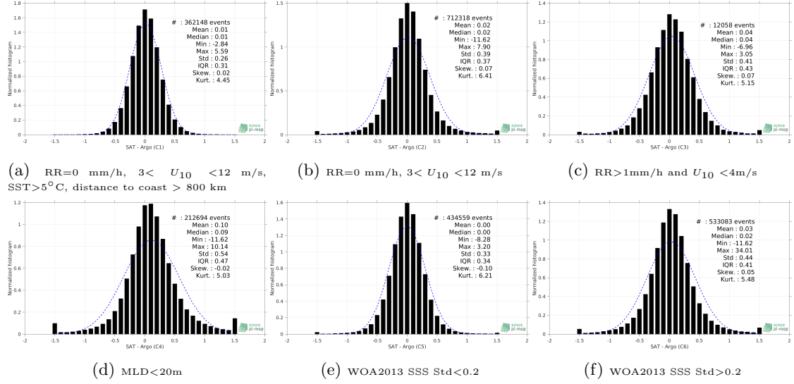
Figure 13: Normalized histogram of \Delta\text{SSS} (SMOS SSS L3 v4 - 9 Days (CATDS-CECOS-LOCEAN) - Argo) for 6 different subdatasets corresponding to: RR=0 mm/h, 3 < U_{10} < 12 m/s, SST>5°C, distance to coast > 800 km (a), RR=0 mm/h, 3 < U_{10} < 12 m/s (b), RR>1mm/h and U_{10} < 4 m/s (c), MLD<20m (d), WOA2013 SSS Std<0.2 (e), WOA2013 SSS Std>0.2 (f).
