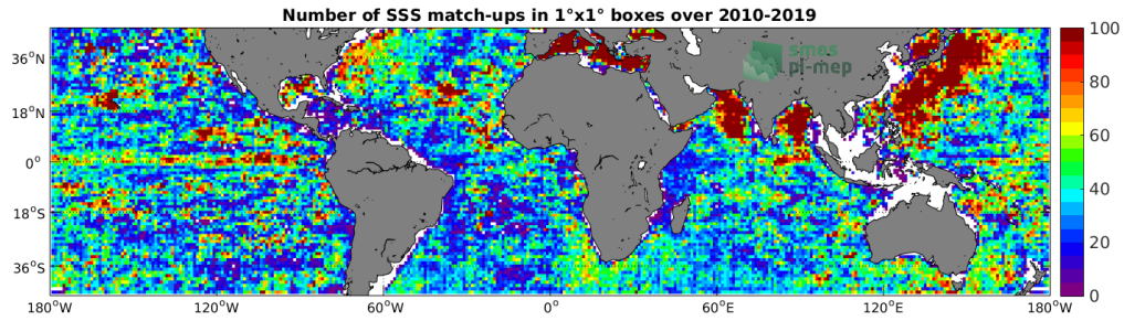
Figure 4: Number of SSS match-ups between Argo SSS and the SMOS SSS L3 v4 - 9 Days (CATDS-CECOS-LOCEAN) SSS product for the Mid-Low Latitudes 45N-45S Pi-MEP region over 1^\circ \times 1^\circ boxes and for the full satellite product period.
