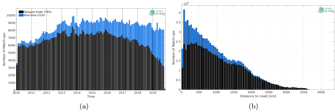
Figure 1: Number of match-ups between Argo and SMOS SSS L3 v4 - 9 Days (CATDS-CECOS-LOCEAN) SSS as a function of time (a) and as function of the distance to coast (b) over the Mid-Low Latitudes 45N-45S Pi-MEP region and for the full satellite product period.
