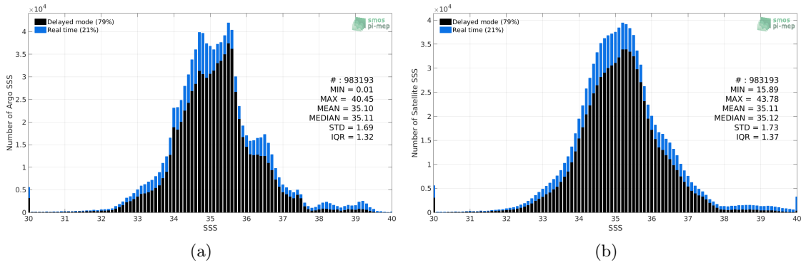
Figure 2: Histograms of SSS from Argo (a) and SMOS SSS L3 v4 - 9 Days (CATDS-CECOS-LOCEAN) (b) considering all match-up pairs per bins of 0.1 over the Mid-Low Latitudes 45N-45S Pi-MEP region and for the full satellite product period.
