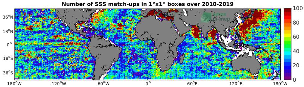
Figure 4: Number of SSS match-ups between Argo SSS and the SMOS-L3-CATDS-CECOS-LOCEAN-V4-9DAYS-25KM SSS product for the Mid-Low Latitudes 45N-45S Pi-MEP region over 1^\circ \times 1^\circ boxes and for the full satellite product period.
