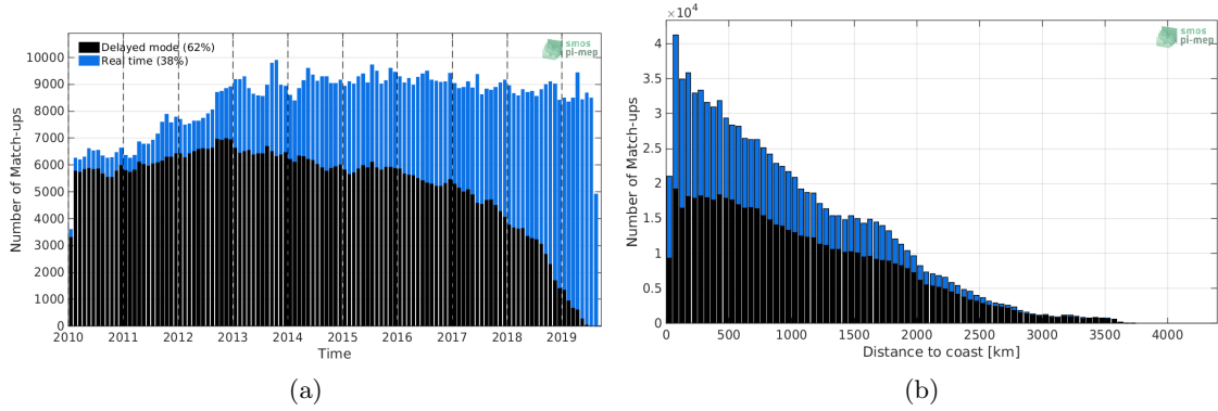
Figure 1: Number of match-ups between Argo and SMOS-L3-CATDS-CECOS-LOCEAN-V4-9DAYS-25KM SSS as a function of time (a) and as function of the distance to coast (b) over the Mid-Low Latitudes 45N-45S Pi-MEP region and for the full satellite product period.
