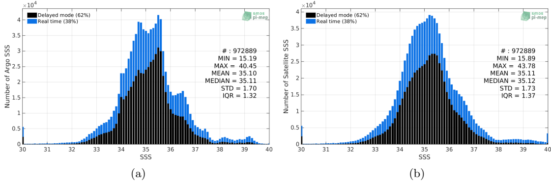
Figure 2: Histograms of SSS from Argo (a) and SMOS-L3-CATDS-CECOS-LOCEAN-V4-9DAYS-25KM (b) considering all match-up pairs per bins of 0.1 over the Mid-Low Latitudes 45N-45S Pi-MEP region and for the full satellite product period.
