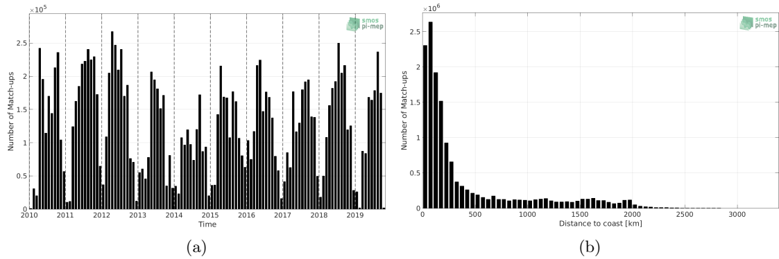
Figure 1: Number of match-ups between TSG-SAMOS and SMOS-L3-CATDS-CECOS-LOCEAN-V4-18DAYS-25KM SSS as a function of time (a) and as function of the distance to coast (b) over the Mid-Low Latitudes 45N-45S Pi-MEP region and for the full satellite product period.
