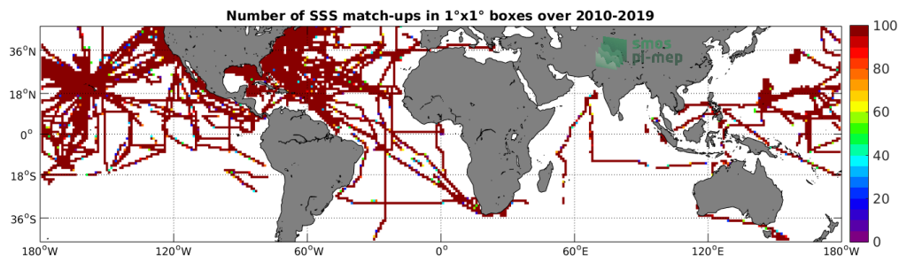
Figure 4: Number of SSS match-ups between TSG-SAMOS SSS and the SMOS-L3-CATDS-CECOS-LOCEAN-V4-18DAYS-25KM SSS product for the Mid-Low Latitudes 45N-45S Pi-MEP region over 1^\circ \times 1^\circ boxes and for the full satellite product period.
