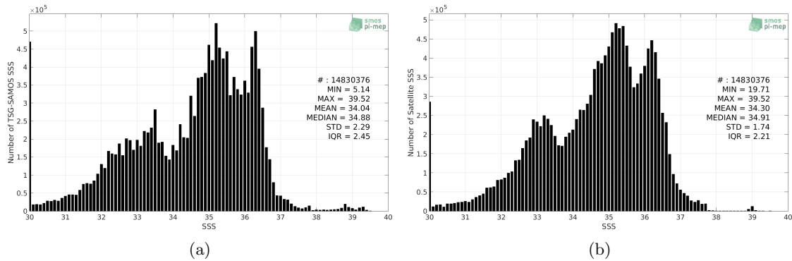
Figure 2: Histograms of SSS from TSG-SAMOS (a) and SMOS-L3-CATDS-CECOS-LOCEAN-V4-18DAYS-25KM (b) considering all match-up pairs per bins of 0.1 over the Mid-Low Latitudes 45N-45S Pi-MEP region and for the full satellite product period.
