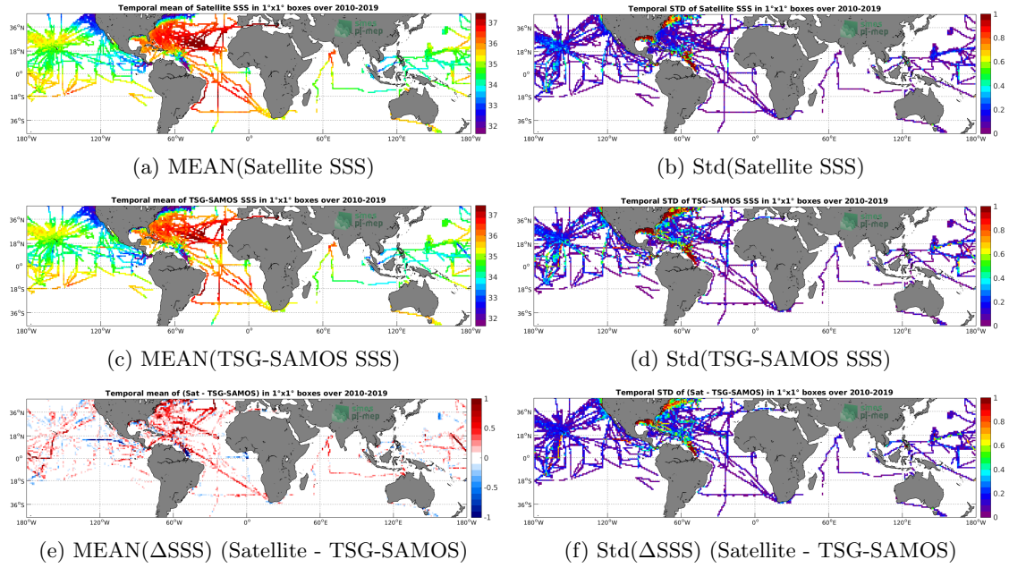
Figure 6: Temporal mean (left) and Std (right) of SSS from SMOS-L3-CATDS-CECOS-LOCEAN-V4-18DAYS-25KM (top), TSG-SAMOS (middle), and of \Delta SSS (Satellite - TSG-SAMOS). Only match-up pairs are used to generate these maps.
