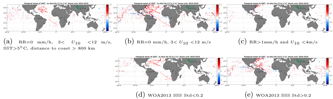
Figure 12: Temporal mean gridded over spatial boxes of size 1^\circ \times 1^\circ of \Delta SSS (SMOS-L3-CATDS-CECOS-LOCEAN-V4-18DAYS-25KM - TSG-SAMOS) for 5 different subdatasets corresponding to:RR=0 mm/h, 3 < U_{10} < 12 m/s, SST >5^\circ C, distance to coast > 800 km (a), RR=0 mm/h, 3 < U_{10} < 12 m/s (b), RR >1 mm/h and U_{10} < 4 m/s (c), WOA2013 SSS Std <0.2 (d), WOA2013 SSS Std >0.2 (e).
