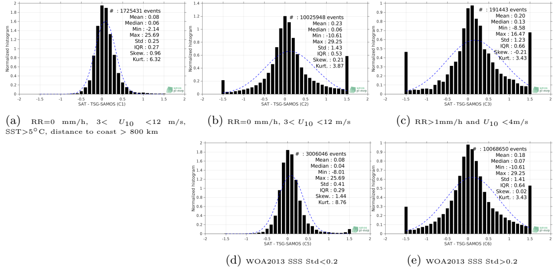
Figure 13: Normalized histogram of \Delta SSS (SMOS-L3-CATDS-CECOS-LOCEAN-V4-18DAYS-25KM - TSG-SAMOS) for 5 different subdatasets corresponding to: RR=0 mm/h, 3 < U_{10} < 12 m/s, SST > 5°C, distance to coast > 800 km (a), RR=0 mm/h, 3 < U_{10} < 12 m/s (b), RR > 1mm/h and U_{10} < 4 m/s (c), WOA2013 SSS Std < 0.2 (d), WOA2013 SSS Std > 0.2 (e).
