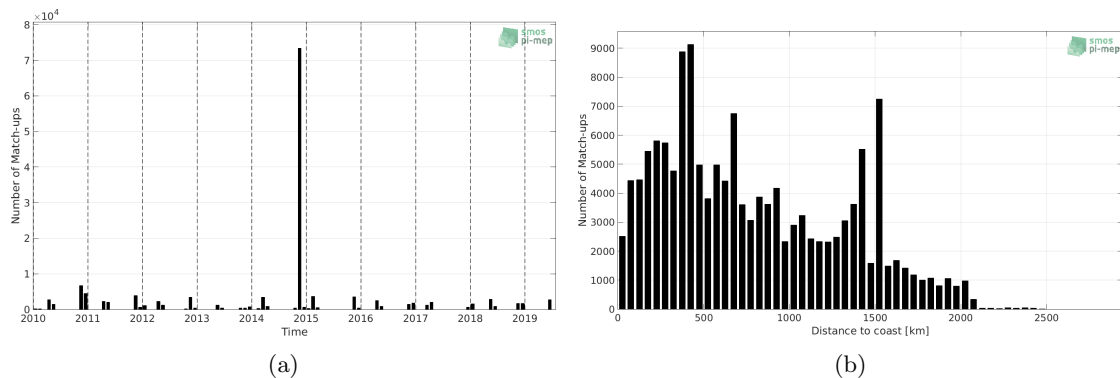
Figure 1: Number of match-ups between TSG-POLARSTERN and SMOS-L3-CATDS-CECOS-LOCEAN-V4-18DAYS-25KM SSS as a function of time (a) and as function of the distance to coast (b) over the Mid-Low Latitudes 45N-45S Pi-MEP region and for the full satellite product period.
