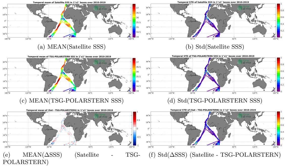
Figure 6: Temporal mean (left) and Std (right) of SSS from SMOS-L3-CATDS-CECOS-LOCEAN-V4-18DAYS-25KM (top), TSG-POLARSTERN (middle), and of \Delta SSS (Satellite - TSG-POLARSTERN). Only match-up pairs are used to generate these maps.
