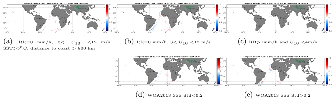
Figure 12: Temporal mean gridded over spatial boxes of size 1^\circ \times 1^\circ of \Delta SSS (SMOS-L3-CATDS-CECOS-LOCEAN-V4-18DAYS-25KM - TSG-POLARSTERN) for 5 different subdatasets corresponding to:RR=0 mm/h, 3 < U_{10} < 12 m/s, SST > 5^\circ\text{C} , distance to coast > 800 km (a), RR=0 mm/h, 3 < U_{10} < 12 m/s (b), RR > 1 mm/h and U_{10} < 4 m/s (c), WOA2013 SSS Std < 0.2 (d), WOA2013 SSS Std > 0.2 (e).
