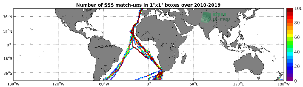
Figure 4: Number of SSS match-ups between TSG-POLARSTERN SSS and the SMOS-L3-CATDS-CECOS-LOCEAN-V4-18DAYS-25KM SSS product for the Mid-Low Latitudes 45N-45S Pi-MEP region over 1^\circ \times 1^\circ boxes and for the full satellite product period.
