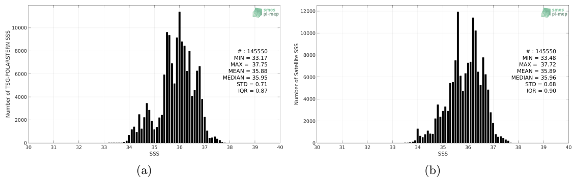
Figure 2: Histograms of SSS from TSG-POLARSTERN (a) and SMOS-L3-CATDS-CECOS-LOCEAN-V4-18DAYS-25KM (b) considering all match-up pairs per bins of 0.1 over the Mid-Low Latitudes 45N-45S Pi-MEP region and for the full satellite product period.
