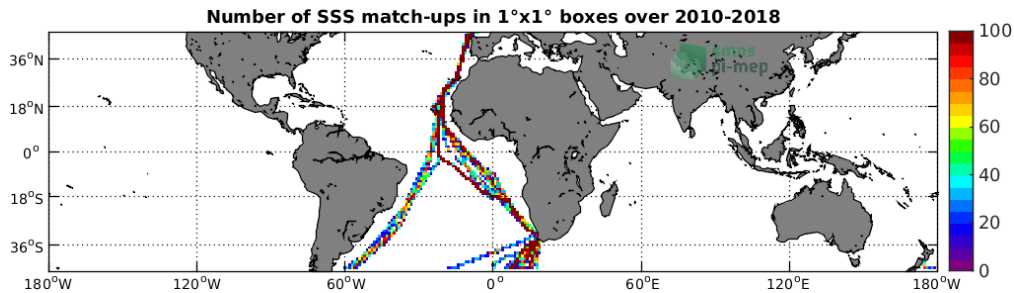
Figure 4: Number of SSS match-ups between TSG-POLARSTERN SSS and the SMOS-L3-CATDS-CECOS-LOCEAN-V4-18DAYS-25KM SSS product for the Mid-Low Latitudes 45N-45S Pi-MEP region over 1°x1° boxes and for the full satellite product period.
