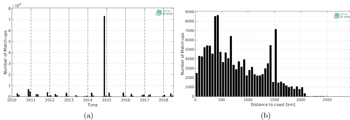
Figure 1: Number of match-ups between TSG-POLARSTERN and SMOS-L3-CATDS-CECOS-LOCEAN-V4-18DAYS-25KM SSS as a function of time (a) and as function of the distance to coast (b) over the Mid-Low Latitudes 45N-45S Pi-MEP region and for the full satellite product period.
