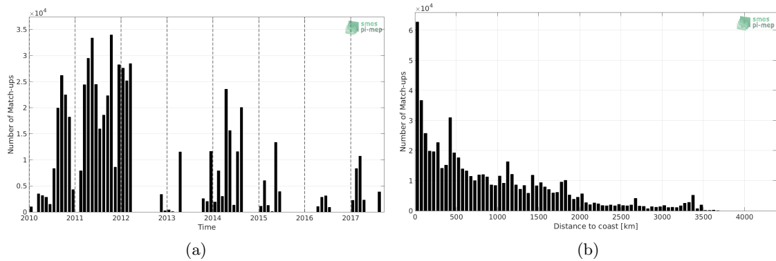
Figure 1: Number of match-ups between TSG-GOSUD-Sailing-ship and SMOS-L3-CATDS-CECOS-LOCEAN-V4-18DAYS-25KM SSS as a function of time (a) and as function of the distance to coast (b) over the Mid-Low Latitudes 45N-45S Pi-MEP region and for the full satellite product period.
