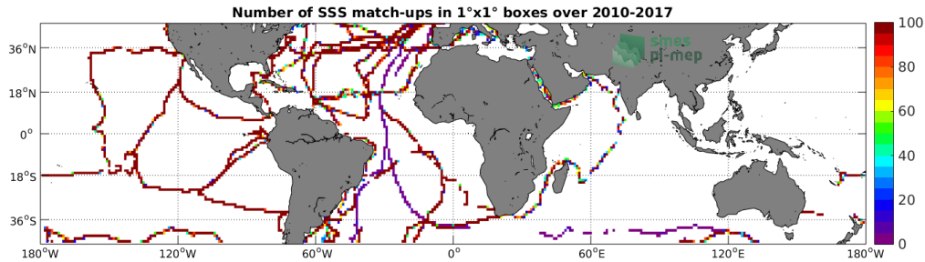
Figure 4: Number of SSS match-ups between TSG-GOSUD-Sailing-ship SSS and the SMOS-L3-CATDS-CECOS-LOCEAN-V4-18DAYS-25KM SSS product for the Mid-Low Latitudes 45N-45S Pi-MEP region over 1°x1° boxes and for the full satellite product period.
