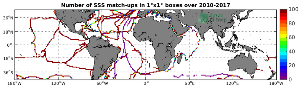
Figure 4: Number of SSS match-ups between TSG-GOSUD-Sailing-ship SSS and the SMOS-L3-CATDS-CECOS-LOCEAN-V4-18DAYS-25KM SSS product for the Mid-Low Latitudes 45N-45S Pi-MEP region over 1^\circ \times 1^\circ boxes and for the full satellite product period.
