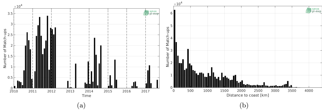
Figure 1: Number of match-ups between TSG-GOSUD-Sailing-ship and SMOS-L3-CATDS-CECOS-LOCEAN-V4-18DAYS-25KM SSS as a function of time (a) and as function of the distance to coast (b) over the Mid-Low Latitudes 45N-45S Pi-MEP region and for the full satellite product period.
