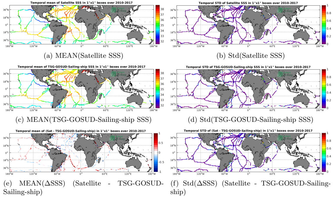
Figure 6: Temporal mean (left) and Std (right) of SSS from SMOS-L3-CATDS-CECOS-LOCEAN-V4-18DAYS-25KM (top), TSG-GOSUD-Sailing-ship (middle), and of \Delta SSS (Satellite - TSG-GOSUD-Sailing-ship). Only match-up pairs are used to generate these maps.
