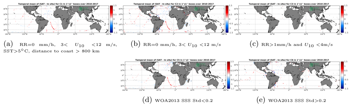
Figure 12: Temporal mean gridded over spatial boxes of size 1^\circ \times 1^\circ of \Delta SSS (SMOS-L3-CATDS-CECOS-LOCEAN-V4-18DAYS-25KM - TSG-GOSUD-Sailing-ship) for 5 different subdatasets corresponding to:RR=0 mm/h, 3 < U_{10} < 12 m/s, SST>5°C, distance to coast > 800 km (a), RR=0 mm/h, 3 < U_{10} < 12 m/s (b), RR>1mm/h and U_{10} < 4 m/s (c), WOA2013 SSS Std<0.2 (d), WOA2013 SSS Std>0.2 (e).
