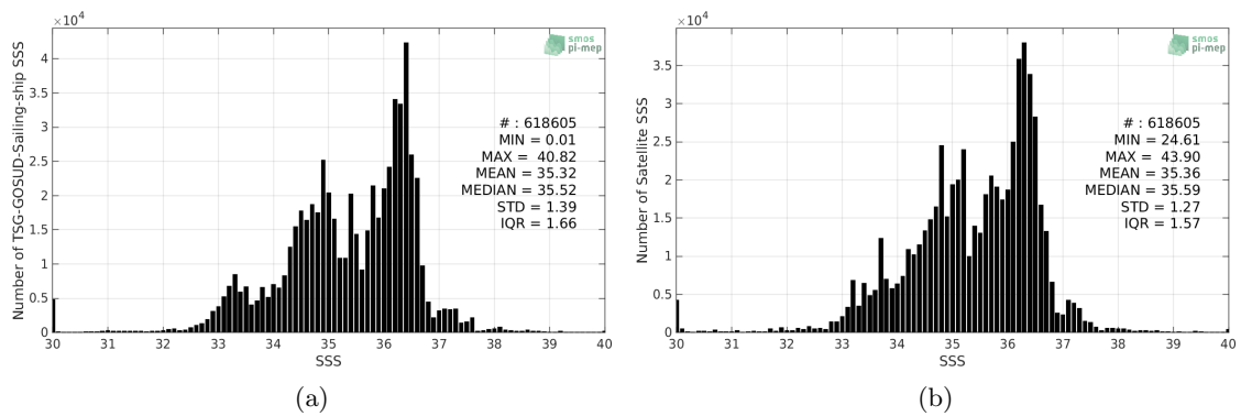
Figure 2: Histograms of SSS from TSG-GOSUD-Sailing-ship (a) and SMOS-L3-CATDS-CECOS-LOCEAN-V4-18DAYS-25KM (b) considering all match-up pairs per bins of 0.1 over the Mid-Low Latitudes 45N-45S Pi-MEP region and for the full satellite product period.
