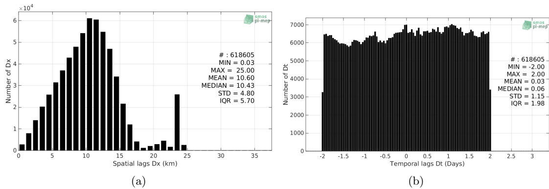
Figure 5: Histograms of the spatial (a) and temporal (b) lags between the time of the TSG-GOSUD-Sailing-ship measurements and the date of the corresponding SMOS-L3-CATDS-CECOS-LOCEAN-V4-18DAYS-25KM SSS product.
