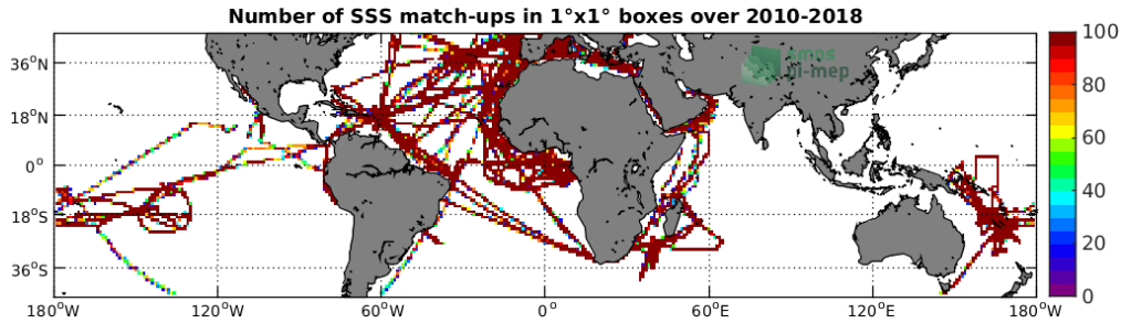
Figure 4: Number of SSS match-ups between TSG-GOSUD-Research-vessel SSS and the SMOS-L3-CATDS-CECOS-LOCEAN-V4-18DAYS-25KM SSS product for the Mid-Low Latitudes 45N-45S Pi-MEP region over 1°x1° boxes and for the full satellite product period.
