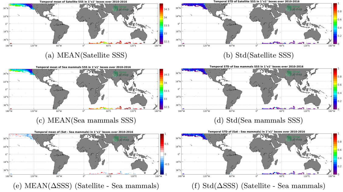
Figure 6: Temporal mean (left) and Std (right) of SSS from SMOS-L3-CATDS-CECOS-LOCEAN-V4-18DAYS-25KM (top), Sea mammals (middle), and of \Delta SSS (Satellite - Sea mammals). Only match-up pairs are used to generate these maps.
