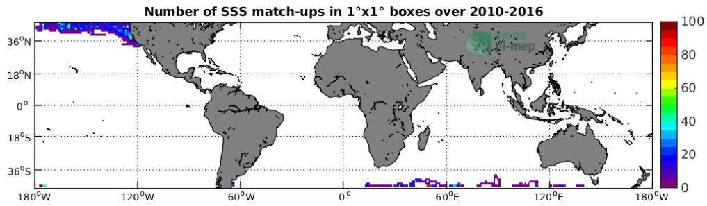
Figure 4: Number of SSS match-ups between Sea mammals SSS and the SMOS-L3-CATDS-CECOS-LOCEAN-V4-18DAYS-25KM SSS product for the Mid-Low Latitudes 45N-45S Pi-MEP region over 1°x1° boxes and for the full satellite product period.
