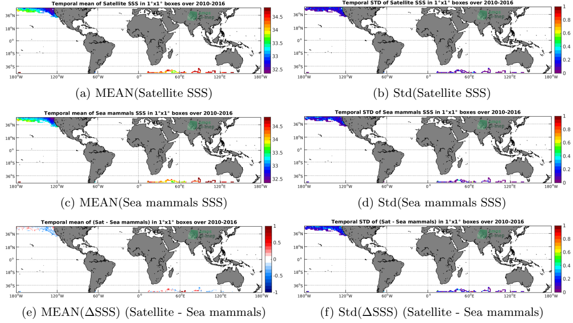
Figure 6: Temporal mean (left) and Std (right) of SSS from SMOS-L3-CATDS-CECOS-LOCEAN-V4-18DAYS-25KM (top), Sea mammals (middle), and of \Delta SSS (Satellite - Sea mammals). Only match-up pairs are used to generate these maps.
