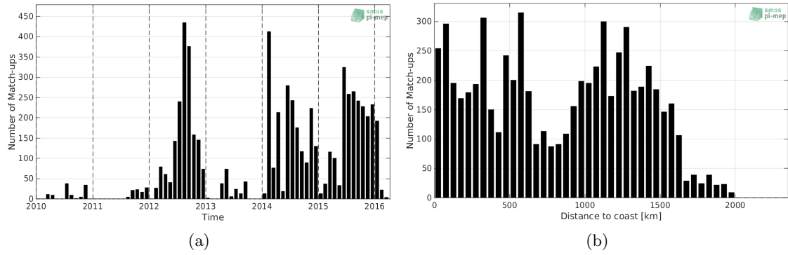
Figure 1: Number of match-ups between Sea mammals and SMOS-L3-CATDS-CECOS-LOCEAN-V4-18DAYS-25KM SSS as a function of time (a) and as function of the distance to coast (b) over the Mid-Low Latitudes 45N-45S Pi-MEP region and for the full satellite product period.
