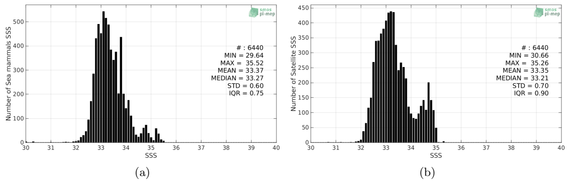
Figure 2: Histograms of SSS from Sea mammals (a) and SMOS-L3-CATDS-CECOS-LOCEAN-V4-18DAYS-25KM (b) considering all match-up pairs per bins of 0.1 over the Mid-Low Latitudes 45N-45S Pi-MEP region and for the full satellite product period.
