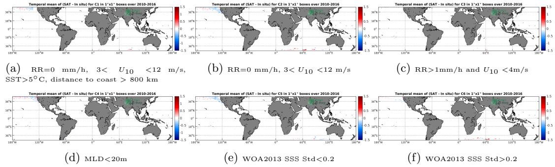
Figure 12: Temporal mean gridded over spatial boxes of size 1^\circ \times 1^\circ of \Delta SSS (SMOS-L3-CATDS-CECOS-LOCEAN-V4-18DAYS-25KM - Sea mammals) for 6 different subdatasets corresponding to: RR=0 mm/h, 3 < U_{10} < 12 m/s, SST >5^\circ C, distance to coast > 800 km (a), RR=0 mm/h, 3 < U_{10} < 12 m/s (b), RR >1 mm/h and U_{10} < 4 m/s (c),MLD <20 m (d),WOA2013 SSS Std <0.2 (e),WOA2013 SSS Std >0.2 (f).
