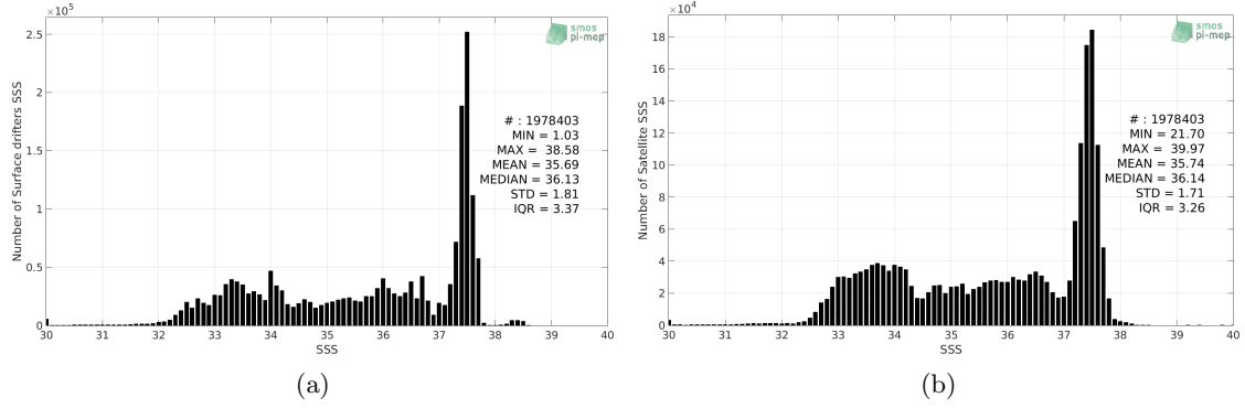
Figure 2: Histograms of SSS from Surface drifters (a) and SMOS SSS L3 v4 - 18 Days (CATDS-CECOS-LOCEAN) (b) considering all match-up pairs per bins of 0.1 over the Mid-Low Latitudes 45N-45S Pi-MEP region and for the full satellite product period.
