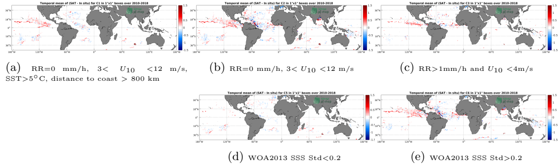
Figure 11: Temporal mean gridded over spatial boxes of size 1^\circ \times 1^\circ of \Delta SSS (SMOS SSS L3 v4 - 18 Days (CATDS-CECOS-LOCEAN) - Surface drifters) for 5 different subdatasets corresponding to: RR=0 mm/h, 3 < U_{10} < 12 m/s, SST > 5^\circ C , distance to coast > 800 km (a), RR=0 mm/h, 3 < U_{10} < 12 m/s (b), RR > 1 mm/h and U_{10} < 4 m/s (c), WOA2013 SSS Std < 0.2 (d), WOA2013 SSS Std > 0.2 (e).
