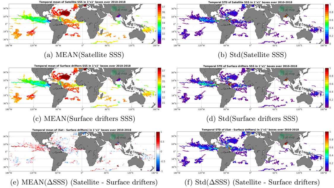
Figure 5: Temporal mean (left) and Std (right) of SSS from SMOS SSS L3 v4 - 18 Days (CATDS-CECOS-LOCEAN) (top), Surface drifters (middle), and of \Delta SSS (Satellite - Surface drifters). Only match-up pairs are used to generate these maps.
