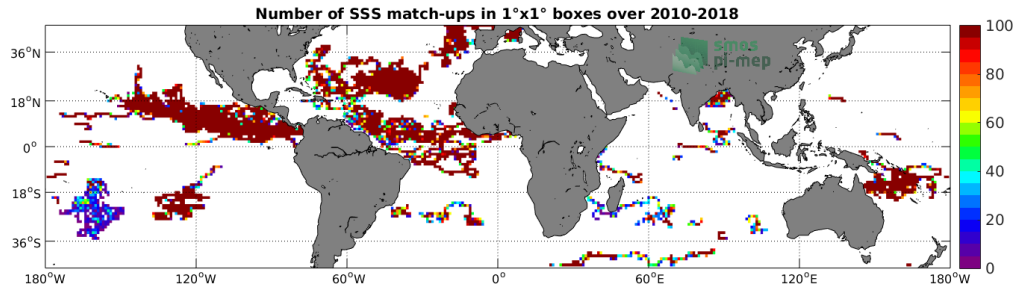
Figure 3: Number of SSS match-ups between Surface drifters SSS and the SMOS SSS L3 v4 - 18 Days (CATDS-CECOS-LOCEAN) SSS product for the Mid-Low Latitudes 45N-45S Pi-MEP region over 1°x1° boxes and for the full satellite product period.
