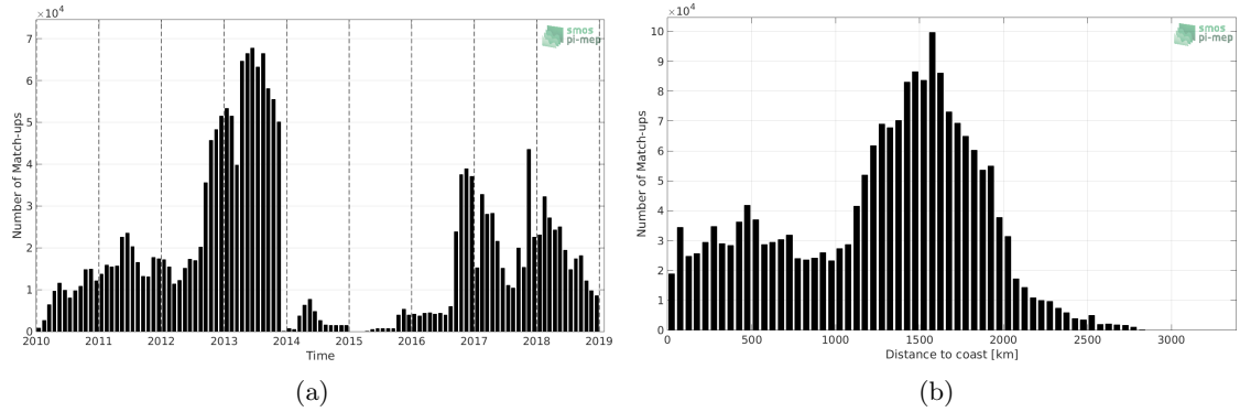
Figure 1: Number of match-ups between Surface drifters and SMOS SSS L3 v4 - 18 Days (CATDS-CECOS-LOCEAN) SSS as a function of time (a) and as function of the distance to coast (b) over the Mid-Low Latitudes 45N-45S Pi-MEP region and for the full satellite product period.
