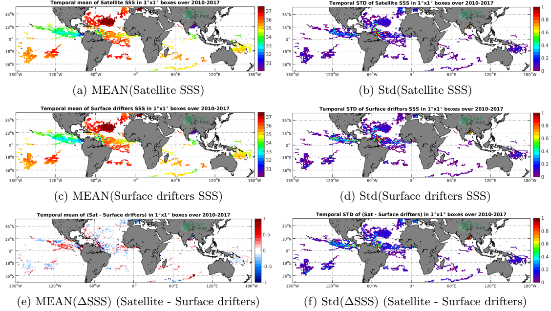
Figure 5: Temporal mean (left) and Std (right) of SSS from SMOS-L3-CATDS-CECOS-LOCEAN-V4-18DAYS-25KM (top), Surface drifters (middle), and of \Delta SSS (Satellite - Surface drifters). Only match-up pairs are used to generate these maps.
