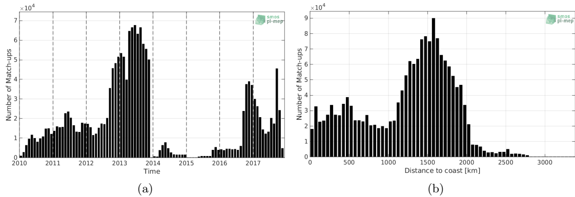
Figure 1: Number of match-ups between Surface drifters and SMOS-L3-CATDS-CECOS-LOCEAN-V4-18DAYS-25KM SSS as a function of time (a) and as function of the distance to coast (b) over the Mid-Low Latitudes 45N-45S Pi-MEP region and for the full satellite product period.
