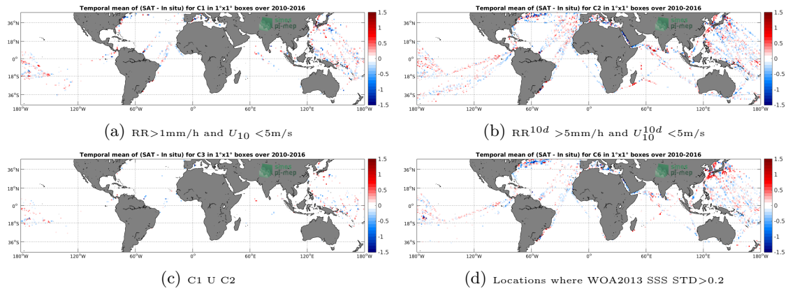
Figure 12: Temporal mean gridded over spatial boxes of size 1^\circ \times 1^\circ of \Delta SSS (SMOS-L3-CATDS-CECOS-LOCEAN-V3-9DAYS-25KM - TSG-LEGOS-DM) for 4 different subdatasets corresponding to: RR > 1\text{mm/h} and U_{10} < 5\text{m/s} (a), RR^{10d} > 5\text{mm/h} and U_{10}^{10d} < 5\text{m/s} (b), C1 U C2 (c), Locations where WOA2013 SSS STD > 0.2 (d).
