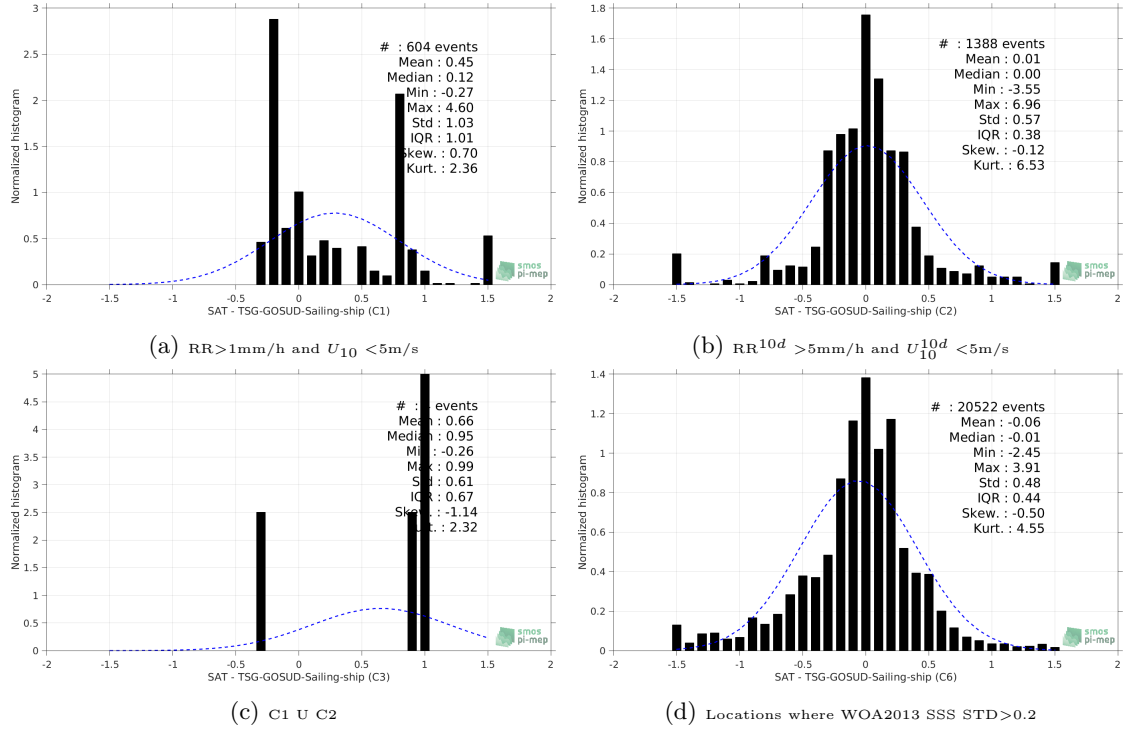
Figure 13: Normalized histogram of \Delta SSS (SMOS-L3-CATDS-CECOS-LOCEAN-V3-9DAYS-25KM - TSG-GOSUD-Sailing-ship) for 6 different subdatasets corresponding to: RR > 1mm/h and U_{10} < 5 m/s (a), RR^{10d} > 5 mm/h and U_{10}^{10d} < 5 m/s (b), C1 U C2 (c), Locations where WOA2013 SSS STD > 0.2 (d).
