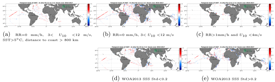
Figure 12: Temporal mean gridded over spatial boxes of size 1^\circ \times 1^\circ of \Delta SSS (SMOS-L3-CATDS-CECOS-LOCEAN-V3-9DAYS-25KM - TSG-GOSUD-Research-vessel) for 5 different subdatasets corresponding to:RR=0 mm/h, 3 < U_{10} < 12 m/s, SST > 5^\circ C , distance to coast > 800 km (a), RR=0 mm/h, 3 < U_{10} < 12 m/s (b), RR >1 mm/h and U_{10} < 4 m/s (c), WOA2013 SSS Std <0.2 (d), WOA2013 SSS Std >0.2 (e).
