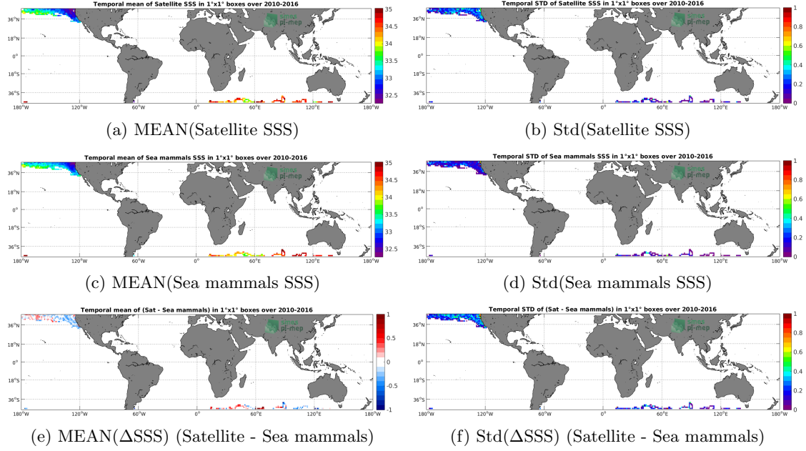
Figure 6: Temporal mean (left) and Std (right) of SSS from SMOS-L3-CATDS-CECOS-LOCEAN-V3-9DAYS-25KM (top), Sea mammals (middle), and of \Delta SSS (Satellite - Sea mammals). Only match-up pairs are used to generate these maps.
