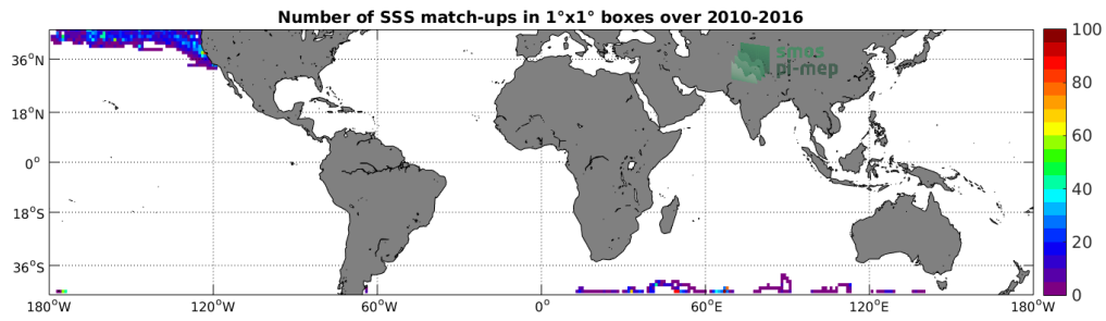
Figure 4: Number of SSS match-ups between Sea mammals SSS and the SMOS-L3-CATDS-CECOS-LOCEAN-V3-9DAYS-25KM SSS product for the Mid-Low Latitudes 45N-45S Pi-MEP region over 1°x1° boxes and for the full satellite product period.
