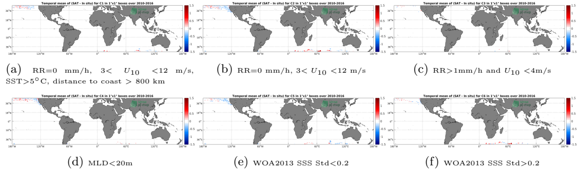
Figure 12: Temporal mean gridded over spatial boxes of size 1^\circ \times 1^\circ of \Delta SSS (SMOS-L3-CATDS-CECOS-LOCEAN-V3-9DAYS-25KM - Sea mammals) for 6 different subdatasets corresponding to: RR=0 mm/h, 3 < U_{10} < 12 m/s, SST >5^\circ\text{C} , distance to coast > 800 km (a), RR=0 mm/h, 3 < U_{10} < 12 m/s (b), RR >1 mm/h and U_{10} < 4 m/s (c),MLD <20 m (d),WOA2013 SSS Std <0.2 (e),WOA2013 SSS Std >0.2 (f).
