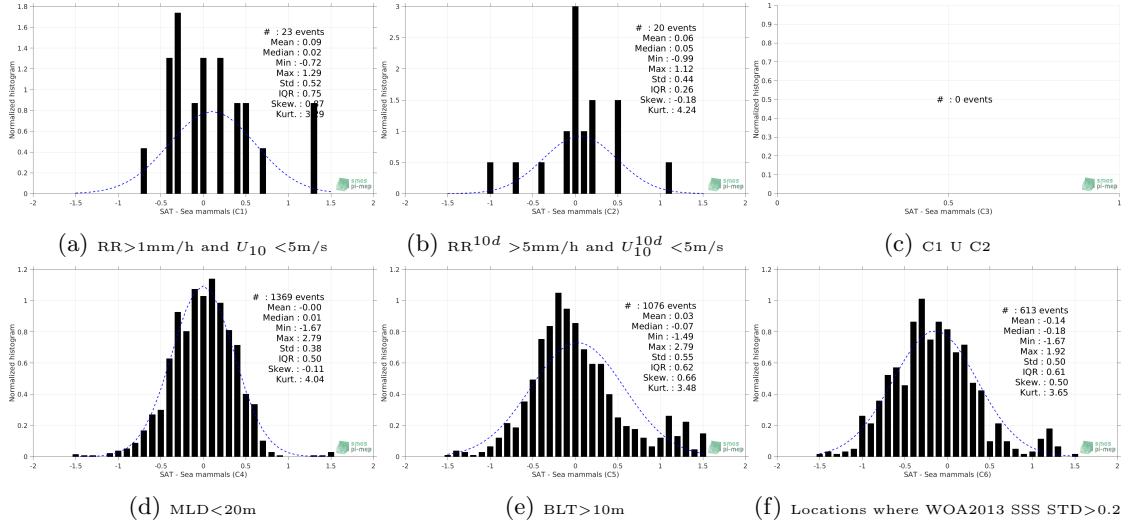
Figure 13: Normalized histogram of \Delta\text{SSS} (SMOS-L3-CATDS-CECOS-LOCEAN-V3-9DAYS-25KM - Sea mammals) for 6 different subdatasets corresponding to: RR>1\text{mm/h} and U_{10}<5\text{m/s} (a), RR^{10d}>5\text{mm/h} and U_{10}^{10d}<5\text{m/s} (b), C1 U C2 (c), MLD<20\text{m} (d), BLT>10\text{m} (e), Locations where WOA2013 SSS STD >0.2 (f).
