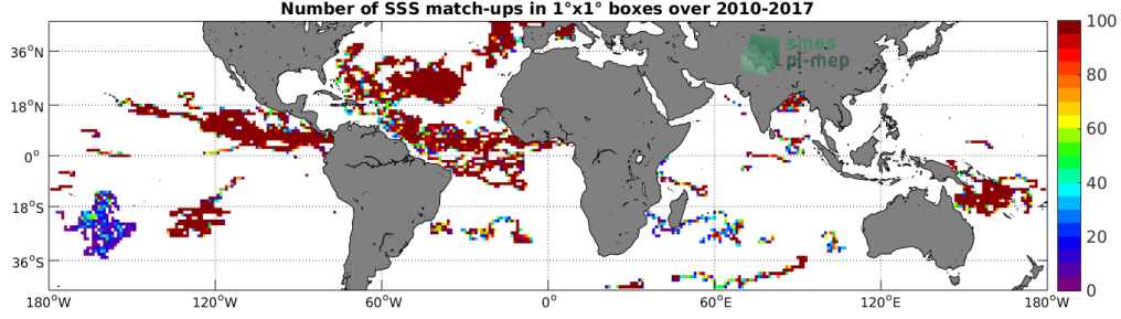
Figure 3: Number of SSS match-ups between Surface drifters SSS and the SMOS-L3-CATDS-CECOS-LOCEAN-V3-9DAYS-25KM SSS product for the Mid-Low Latitudes 45N-45S Pi-MEP region over 1°x1° boxes and for the full satellite product period.
