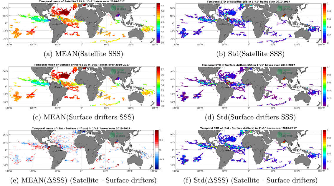
Figure 5: Temporal mean (left) and Std (right) of SSS from SMOS-L3-CATDS-CECOS-LOCEAN-V3-9DAYS-25KM (top), Surface drifters (middle), and of \Delta SSS (Satellite - Surface drifters). Only match-up pairs are used to generate these maps.
