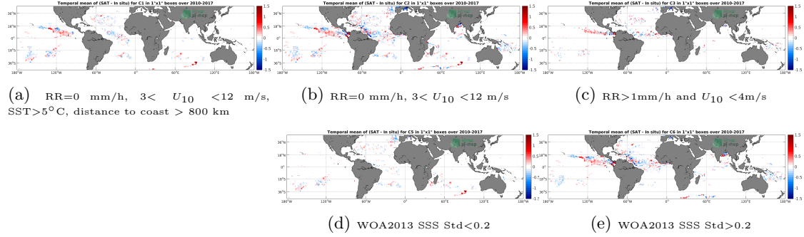
Figure 11: Temporal mean gridded over spatial boxes of size 1^\circ \times 1^\circ of \Delta SSS (SMOS-L3-CATDS-CECOS-LOCEAN-V3-9DAYS-25KM - Surface drifters) for 5 different subdatasets corresponding to: RR=0 mm/h, 3 < U_{10} < 12 m/s, SST > 5^\circ C , distance to coast > 800 km (a), RR=0 mm/h, 3 < U_{10} < 12 m/s (b), RR > 1 mm/h and U_{10} < 4 m/s (c), WOA2013 SSS Std < 0.2 (d), WOA2013 SSS Std > 0.2 (e).
