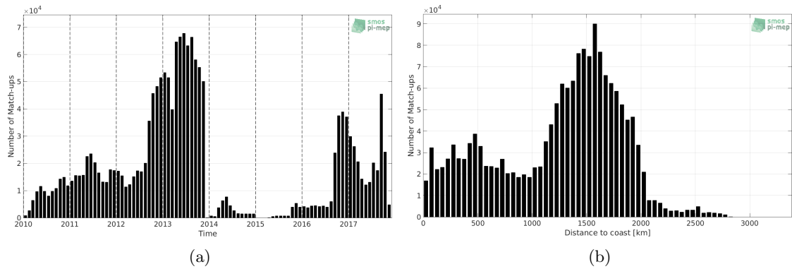
Figure 1: Number of match-ups between Surface drifters and SMOS-L3-CATDS-CECOS-LOCEAN-V3-9DAYS-25KM SSS as a function of time (a) and as function of the distance to coast (b) over the Mid-Low Latitudes 45N-45S Pi-MEP region and for the full satellite product period.
