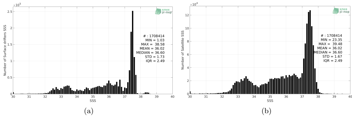
Figure 2: Histograms of SSS from Surface drifters (a) and SMOS-L3-CATDS-CECOS-LOCEAN-V3-9DAYS-25KM (b) considering all match-up pairs per bins of 0.1 over the Mid-Low Latitudes 45N-45S Pi-MEP region and for the full satellite product period.
