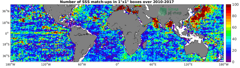
Figure 4: Number of SSS match-ups between Argo SSS and the SMOS-L3-CATDS-CECOS-LOCEAN-V3-9DAYS-25KM SSS product for the Mid-Low Latitudes 45N-45S Pi-MEP region over 1°x1° boxes and for the full satellite product period.
