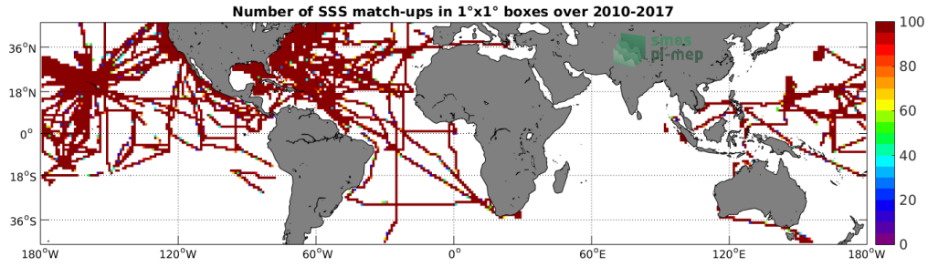
Figure 4: Number of SSS match-ups between TSG-SAMOS SSS and the SMOS-L3-CATDS-CECOS-LOCEAN-V3-18DAYS-25KM SSS product for the Mid-Low Latitudes 45N-45S Pi-MEP region over 1°x1° boxes and for the full satellite product period.
