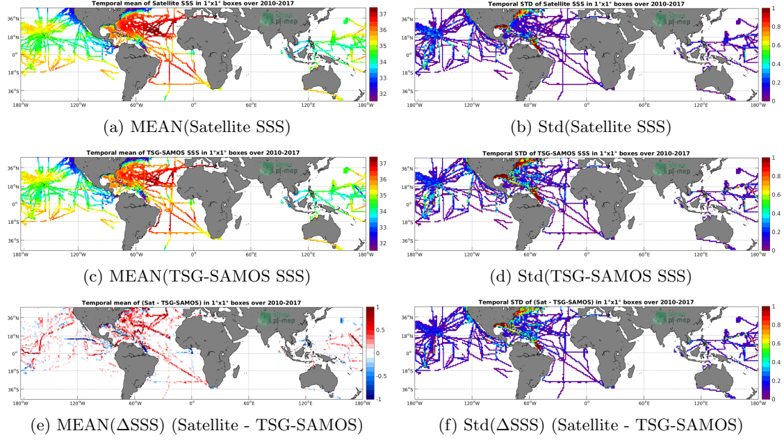
Figure 6: Temporal mean (left) and Std (right) of SSS from SMOS-L3-CATDS-CECOS-LOCEAN-V3-18DAYS-25KM (top), TSG-SAMOS (middle), and of \Delta SSS (Satellite - TSG-SAMOS). Only match-up pairs are used to generate these maps.
