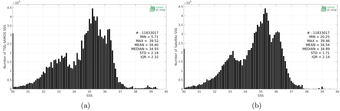
Figure 2: Histograms of SSS from TSG-SAMOS (a) and SMOS-L3-CATDS-CECOS-LOCEAN-V3-18DAYS-25KM (b) considering all match-up pairs per bins of 0.1 over the Mid-Low Latitudes 45N-45S Pi-MEP region and for the full satellite product period.
