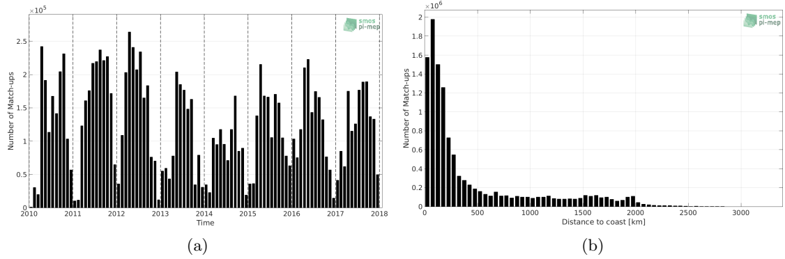
Figure 1: Number of match-ups between TSG-SAMOS and SMOS-L3-CATDS-CECOS-LOCEAN-V3-18DAYS-25KM SSS as a function of time (a) and as function of the distance to coast (b) over the Mid-Low Latitudes 45N-45S Pi-MEP region and for the full satellite product period.
