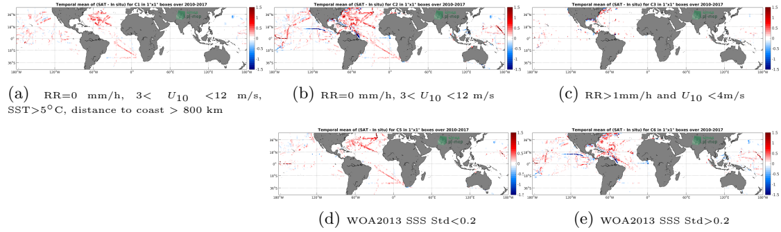
Figure 12: Temporal mean gridded over spatial boxes of size 1^\circ \times 1^\circ of \Delta SSS (SMOS-L3-CATDS-CECOS-LOCEAN-V3-18DAYS-25KM - TSG-SAMOS) for 5 different subdatasets corresponding to: RR=0 mm/h, 3 < U_{10} < 12 m/s, SST > 5^\circ C , distance to coast > 800 km (a), RR=0 mm/h, 3 < U_{10} < 12 m/s (b), RR > 1 mm/h and U_{10} < 4 m/s (c), WOA2013 SSS Std < 0.2 (d), WOA2013 SSS Std > 0.2 (e).
