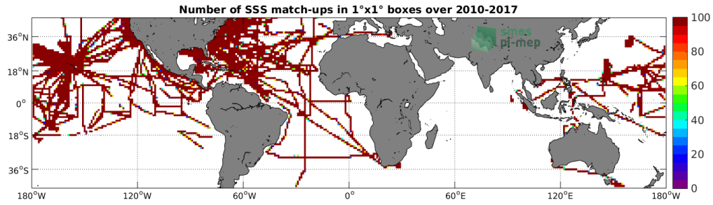
Figure 4: Number of SSS match-ups between TSG-SAMOS SSS and the SMOS-L3-CATDS-CECOS-LOCEAN-V3-18DAYS-25KM SSS product for the Mid-Low Latitudes 45N-45S Pi-MEP region over 1^\circ \times 1^\circ boxes and for the full satellite product period.
