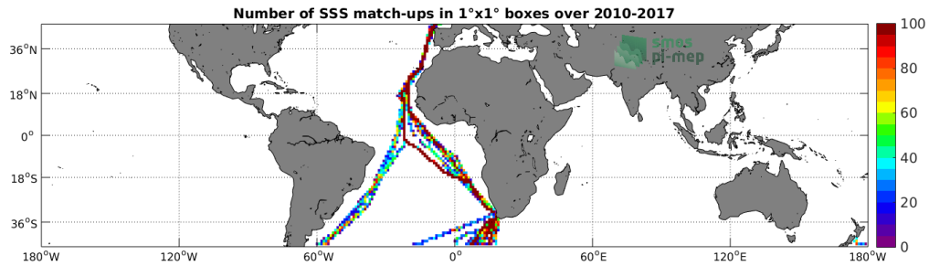
Figure 4: Number of SSS match-ups between TSG-POLARSTERN SSS and the SMOS-L3-CATDS-CECOS-LOCEAN-V3-18DAYS-25KM SSS product for the Mid-Low Latitudes 45N-45S Pi-MEP region over 1^\circ \times 1^\circ boxes and for the full satellite product period.
