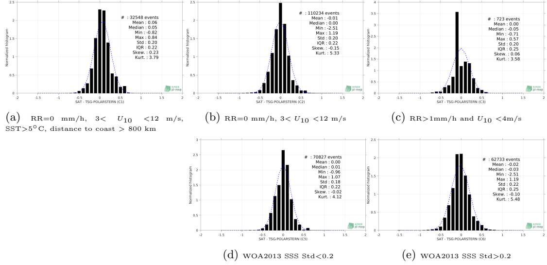
Figure 13: Normalized histogram of \Delta SSS (SMOS-L3-CATDS-CECOS-LOCEAN-V3-18DAYS-25KM - TSG-POLARSTERN) for 5 different subdatasets corresponding to: RR=0 mm/h, 3 < U_{10} < 12 m/s, SST>5°C, distance to coast > 800 km (a), RR=0 mm/h, 3 < U_{10} < 12 m/s (b), RR>1mm/h and U_{10} < 4 m/s (c), WOA2013 SSS Std<0.2 (d), WOA2013 SSS Std>0.2 (e).
