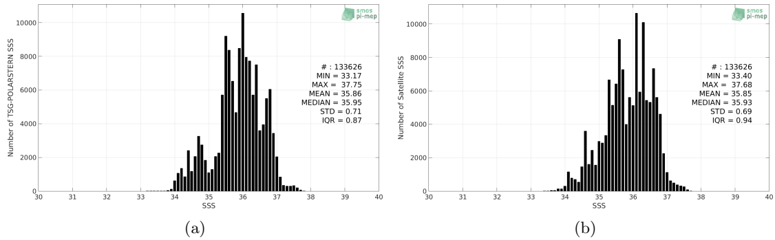
Figure 2: Histograms of SSS from TSG-POLARSTERN (a) and SMOS-L3-CATDS-CECOS-LOCEAN-V3-18DAYS-25KM (b) considering all match-up pairs per bins of 0.1 over the Mid-Low Latitudes 45N-45S Pi-MEP region and for the full satellite product period.
