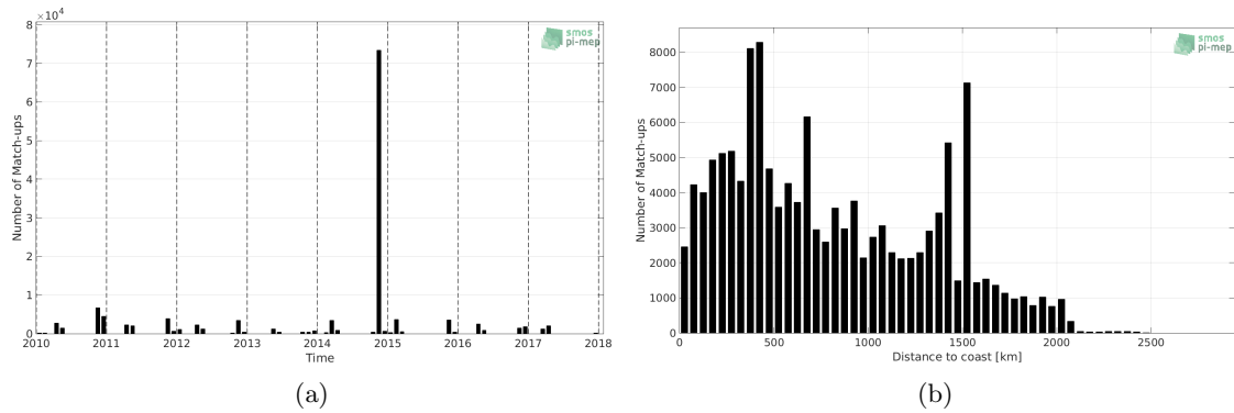
Figure 1: Number of match-ups between TSG-POLARSTERN and SMOS-L3-CATDS-CECOS-LOCEAN-V3-18DAYS-25KM SSS as a function of time (a) and as function of the distance to coast (b) over the Mid-Low Latitudes 45N-45S Pi-MEP region and for the full satellite product period.
