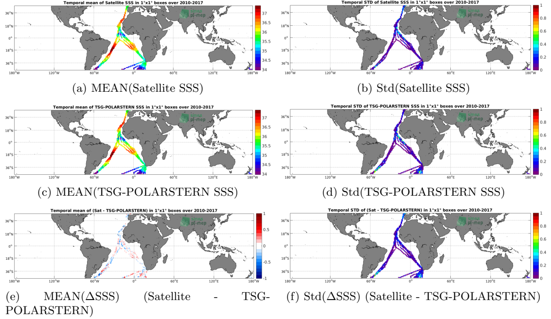
Figure 6: Temporal mean (left) and Std (right) of SSS from SMOS-L3-CATDS-CECOS-LOCEAN-V3-18DAYS-25KM (top), TSG-POLARSTERN (middle), and of \Delta SSS (Satellite - TSG-POLARSTERN). Only match-up pairs are used to generate these maps.
