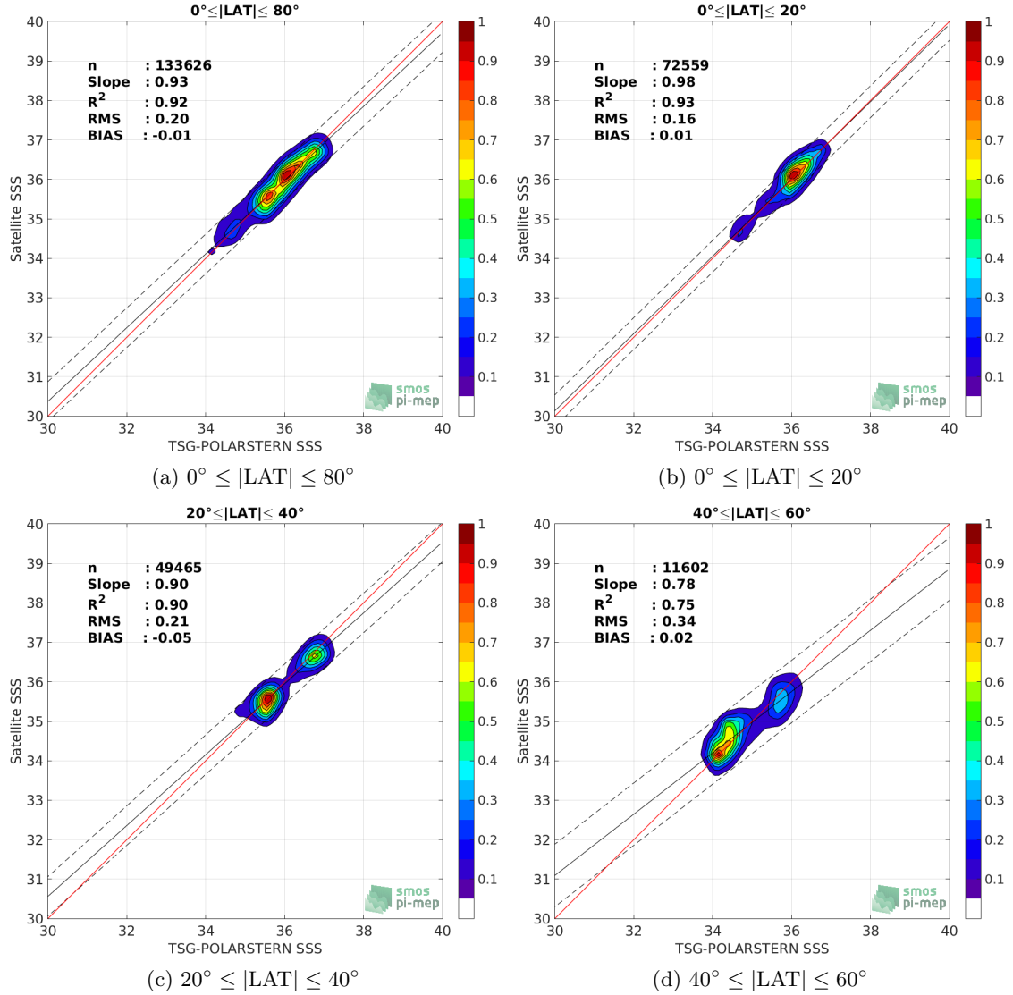
Figure 9: Contour maps of the concentration of SMOS-L3-CATDS-CECOS-LOCEAN-V3-18DAYS-25KM SSS (y-axis) versus TSG-POLARSTERN SSS (x-axis) at match-up pairs for different latitude bands. For each plot, the red line shows x=y . The black thin and dashed lines indicate a linear fit through the data cloud and the \pm 95\% confidence levels, respectively. The number match-up pairs n , the slope and R^2 coefficient of the linear fit, the root mean square (RMS) and the mean bias between satellite and in situ data are indicated for each latitude band in each plots.
