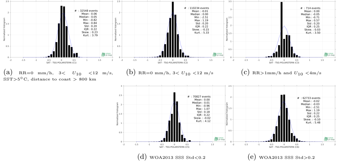
Figure 13: Normalized histogram of \Delta SSS (SMOS-L3-CATDS-CECOS-LOCEAN-V3-18DAYS-25KM - TSG-POLARSTERN) for 5 different subdatasets corresponding to: RR=0 mm/h, 3 < U_{10} < 12 m/s, SST > 5°C, distance to coast > 800 km (a), RR=0 mm/h, 3 < U_{10} < 12 m/s (b), RR > 1mm/h and U_{10} < 4 m/s (c), WOA2013 SSS Std < 0.2 (d), WOA2013 SSS Std > 0.2 (e).
