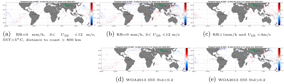
Figure 12: Temporal mean gridded over spatial boxes of size 1^\circ \times 1^\circ of \Delta SSS (SMOS-L3-CATDS-CECOS-LOCEAN-V3-18DAYS-25KM - TSG-LEGOS-DM) for 5 different subdatasets corresponding to: RR=0 mm/h, 3 < U_{10} < 12 m/s, SST > 5^\circ\text{C} , distance to coast > 800 km (a), RR=0 mm/h, 3 < U_{10} < 12 m/s (b), RR > 1 mm/h and U_{10} < 4 m/s (c), WOA2013 SSS Std < 0.2 (d), WOA2013 SSS Std > 0.2 (e).
