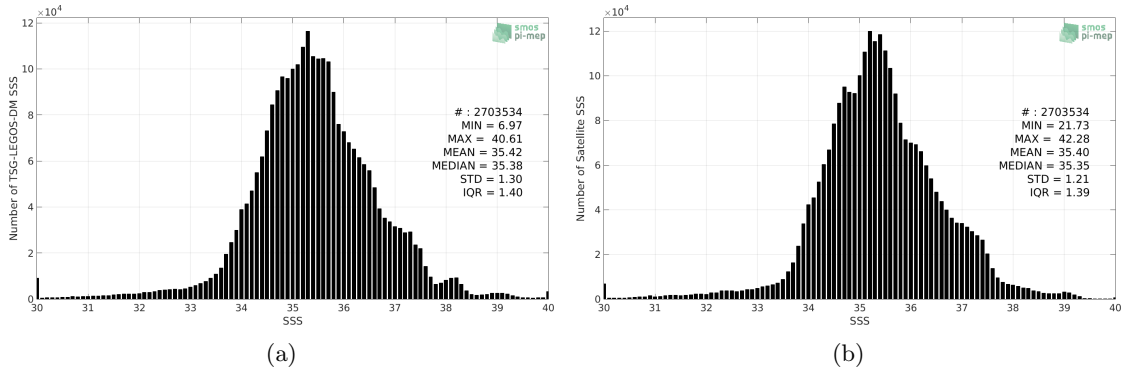
Figure 2: Histograms of SSS from TSG-LEGOS-DM (a) and SMOS-L3-CATDS-CECOS-LOCEAN-V3-18DAYS-25KM (b) considering all match-up pairs per bins of 0.1 over the Mid-Low Latitudes 45N-45S Pi-MEP region and for the full satellite product period.
