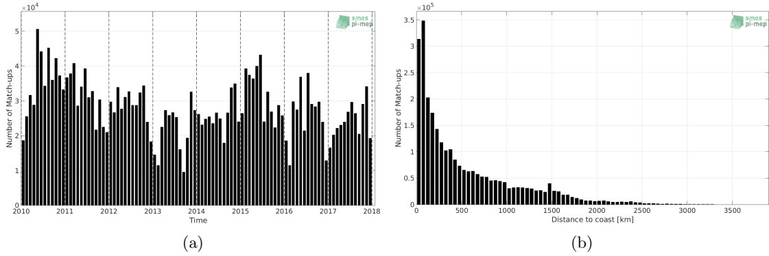
Figure 1: Number of match-ups between TSG-LEGOS-DM and SMOS-L3-CATDS-CECOS-LOCEAN-V3-18DAYS-25KM SSS as a function of time (a) and as function of the distance to coast (b) over the Mid-Low Latitudes 45N-45S Pi-MEP region and for the full satellite product period.
