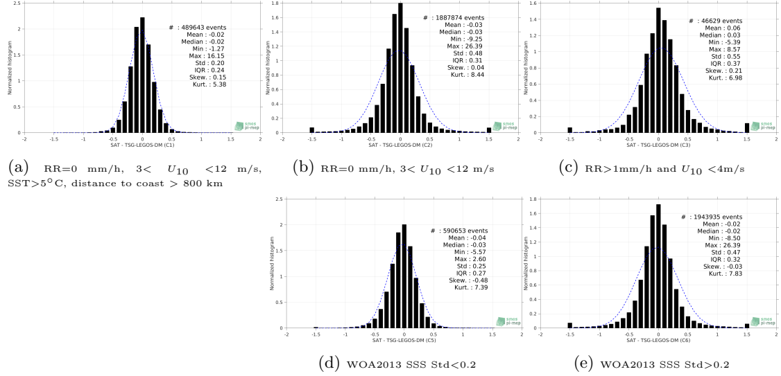
Figure 13: Normalized histogram of \Delta SSS (SMOS-L3-CATDS-CECOS-LOCEAN-V3-18DAYS-25KM - TSG-LEGOS-DM) for 5 different subdatasets corresponding to: RR=0 mm/h, 3 < U_{10} < 12 m/s, SST > 5°C, distance to coast > 800 km (a), RR=0 mm/h, 3 < U_{10} < 12 m/s (b), RR > 1mm/h and U_{10} < 4 m/s (c), WOA2013 SSS Std < 0.2 (d), WOA2013 SSS Std > 0.2 (e).
