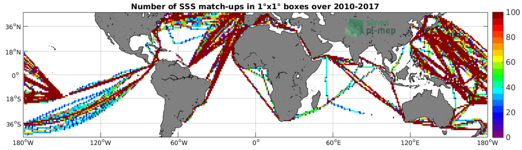
Figure 4: Number of SSS match-ups between TSG-LEGOS-DM SSS and the SMOS-L3-CATDS-CECOS-LOCEAN-V3-18DAYS-25KM SSS product for the Mid-Low Latitudes 45N-45S Pi-MEP region over 1°x1° boxes and for the full satellite product period.
