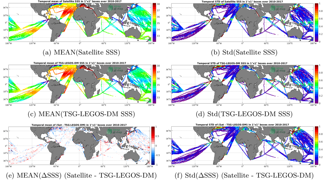
Figure 6: Temporal mean (left) and Std (right) of SSS from SMOS-L3-CATDS-CECOS-LOCEAN-V3-18DAYS-25KM (top), TSG-LEGOS-DM (middle), and of \Delta SSS (Satellite - TSG-LEGOS-DM). Only match-up pairs are used to generate these maps.
