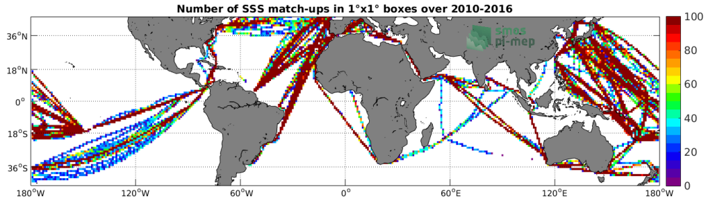
Figure 4: Number of SSS match-ups between TSG-LEGOS-DM SSS and the SMOS-L3-CATDS-CECOS-LOCEAN-V3-18DAYS-25KM SSS product for the Mid-Low Latitudes 45N-45S Pi-MEP region over 1^\circ \times 1^\circ boxes and for the full satellite product period.
