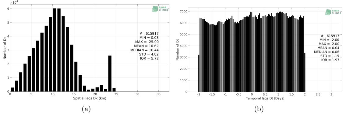
Figure 5: Histograms of the spatial (a) and temporal (b) lags between the time of the TSG-GOSUD-Sailing-ship measurements and the date of the corresponding SMOS-L3-CATDS-CECOS-LOCEAN-V3-18DAYS-25KM SSS product.
