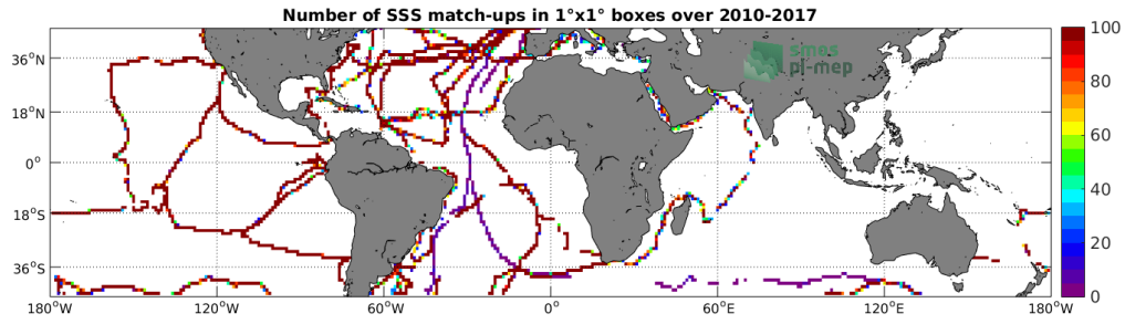
Figure 4: Number of SSS match-ups between TSG-GOSUD-Sailing-ship SSS and the SMOS-L3-CATDS-CECOS-LOCEAN-V3-18DAYS-25KM SSS product for the Mid-Low Latitudes 45N-45S Pi-MEP region over 1^\circ \times 1^\circ boxes and for the full satellite product period.
