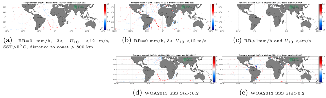
Figure 12: Temporal mean gridded over spatial boxes of size 1^\circ \times 1^\circ of \Delta SSS (SMOS-L3-CATDS-CECOS-LOCEAN-V3-18DAYS-25KM - TSG-GOSUD-Sailing-ship) for 5 different subdatasets corresponding to: RR=0 mm/h, 3 < U_{10} < 12 m/s, SST > 5^\circ C , distance to coast > 800 km (a), RR=0 mm/h, 3 < U_{10} < 12 m/s (b), RR > 1 mm/h and U_{10} < 4 m/s (c), WOA2013 SSS Std < 0.2 (d), WOA2013 SSS Std > 0.2 (e).
