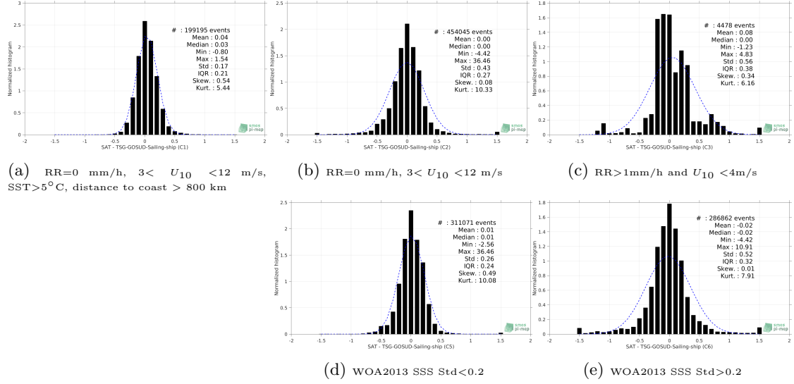
Figure 13: Normalized histogram of \Delta SSS (SMOS-L3-CATDS-CECOS-LOCEAN-V3-18DAYS-25KM - TSG-GOSUD-Sailing-ship) for 5 different subdatasets corresponding to: RR=0 mm/h, 3 < U_{10} < 12 m/s, SST > 5^\circ\text{C} , distance to coast > 800 km (a), RR=0 mm/h, 3 < U_{10} < 12 m/s (b), RR > 1\text{mm/h} and U_{10} < 4\text{m/s} (c), WOA2013 SSS Std < 0.2 (d), WOA2013 SSS Std > 0.2 (e).
