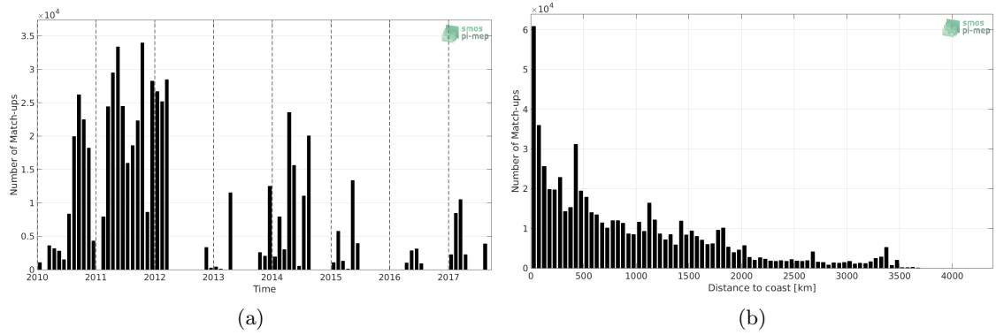
Figure 1: Number of match-ups between TSG-GOSUD-Sailing-ship and SMOS-L3-CATDS-CECOS-LOCEAN-V3-18DAYS-25KM SSS as a function of time (a) and as function of the distance to coast (b) over the Mid-Low Latitudes 45N-45S Pi-MEP region and for the full satellite product period.
