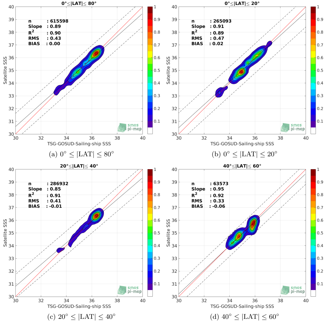
Figure 9: Contour maps of the concentration of SMOS-L3-CATDS-CECOS-LOCEAN-V3-18DAYS-25KM SSS (y-axis) versus TSG-GOSUD-Sailing-ship SSS (x-axis) at match-up pairs for different latitude bands. For each plot, the red line shows x=y . The black thin and dashed lines indicate a linear fit through the data cloud and the \pm 95\% confidence levels, respectively. The number match-up pairs n , the slope and R^2 coefficient of the linear fit, the root mean square (RMS) and the mean bias between satellite and in situ data are indicated for each latitude band in each plots.
