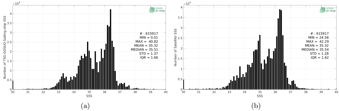
Figure 2: Histograms of SSS from TSG-GOSUD-Sailing-ship (a) and SMOS-L3-CATDS-CECOS-LOCEAN-V3-18DAYS-25KM (b) considering all match-up pairs per bins of 0.1 over the Mid-Low Latitudes 45N-45S Pi-MEP region and for the full satellite product period.
