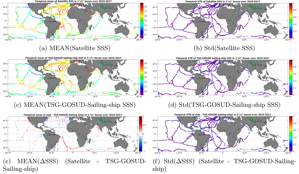
Figure 6: Temporal mean (left) and Std (right) of SSS from SMOS-L3-CATDS-CECOS-LOCEAN-V3-18DAYS-25KM (top), TSG-GOSUD-Sailing-ship (middle), and of \Delta SSS (Satellite - TSG-GOSUD-Sailing-ship). Only match-up pairs are used to generate these maps.
