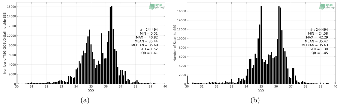
Figure 2: Histograms of SSS from TSG-GOSUD-Sailing-ship (a) and SMOS-L3-CATDS-CECOS-LOCEAN-V3-18DAYS-25KM (b) considering all match-up pairs per bins of 0.1 over the Mid-Low Latitudes 45N-45S Pi-MEP region and for the full satellite product period.
