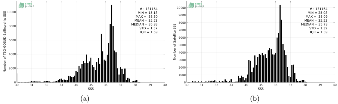
Figure 2: Histograms of SSS from TSG-GOSUD-Sailing-ship (a) and SMOS-L3-CATDS-CECOS-LOCEAN-V3-18DAYS-25KM (b) considering all match-up pairs per bins of 0.1 over the Mid-Low Latitudes 45N-45S Pi-MEP region and for the full satellite product period.
