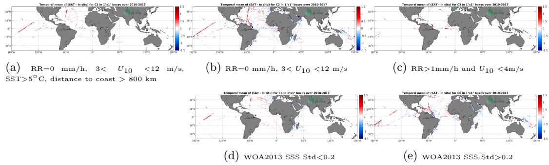
Figure 12: Temporal mean gridded over spatial boxes of size 1^\circ \times 1^\circ of \Delta SSS (SMOS-L3-CATDS-CECOS-LOCEAN-V3-18DAYS-25KM - TSG-GOSUD-Research-vessel) for 5 different subdatasets corresponding to: RR=0 mm/h, 3 < U_{10} < 12 m/s, SST > 5^\circ C , distance to coast > 800 km (a), RR=0 mm/h, 3 < U_{10} < 12 m/s (b), RR > 1 mm/h and U_{10} < 4 m/s (c), WOA2013 SSS Std < 0.2 (d), WOA2013 SSS Std > 0.2 (e).
