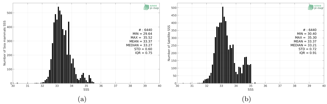
Figure 2: Histograms of SSS from Sea mammals (a) and SMOS-L3-CATDS-CECOS-LOCEAN-V3-18DAYS-25KM (b) considering all match-up pairs per bins of 0.1 over the Mid-Low Latitudes 45N-45S Pi-MEP region and for the full satellite product period.
