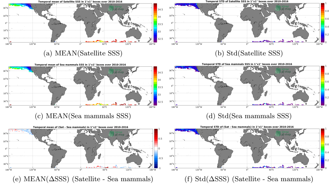
Figure 6: Temporal mean (left) and Std (right) of SSS from SMOS-L3-CATDS-CECOS-LOCEAN-V3-18DAYS-25KM (top), Sea mammals (middle), and of \Delta SSS (Satellite - Sea mammals). Only match-up pairs are used to generate these maps.
