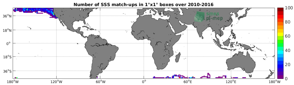
Figure 4: Number of SSS match-ups between Sea mammals SSS and the SMOS-L3-CATDS-CECOS-LOCEAN-V3-18DAYS-25KM SSS product for the Mid-Low Latitudes 45N-45S Pi-MEP region over 1°x1° boxes and for the full satellite product period.
