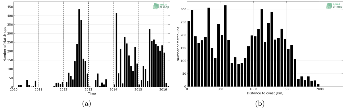
Figure 1: Number of match-ups between Sea mammals and SMOS-L3-CATDS-CECOS-LOCEAN-V3-18DAYS-25KM SSS as a function of time (a) and as function of the distance to coast (b) over the Mid-Low Latitudes 45N-45S Pi-MEP region and for the full satellite product period.
