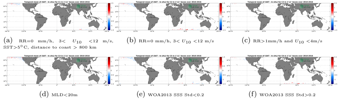
Figure 12: Temporal mean gridded over spatial boxes of size 1^\circ \times 1^\circ of \Delta SSS (SMOS-L3-CATDS-CECOS-LOCEAN-V3-18DAYS-25KM - Sea mammals) for 6 different subdatasets corresponding to: RR=0 mm/h, 3 < U_{10} < 12 m/s, SST > 5^\circ C , distance to coast > 800 km (a), RR=0 mm/h, 3 < U_{10} < 12 m/s (b), RR > 1 mm/h and U_{10} < 4 m/s (c), MLD < 20 m (d), WOA2013 SSS Std < 0.2 (e), WOA2013 SSS Std > 0.2 (f).
