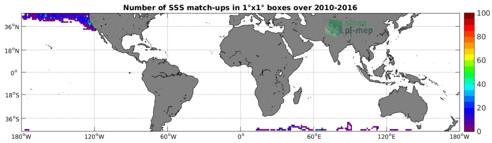
Figure 4: Number of SSS match-ups between Sea mammals SSS and the SMOS-L3-CATDS-CECOS-LOCEAN-V3-18DAYS-25KM SSS product for the Mid-Low Latitudes 45N-45S Pi-MEP region over 1^\circ \times 1^\circ boxes and for the full satellite product period.
