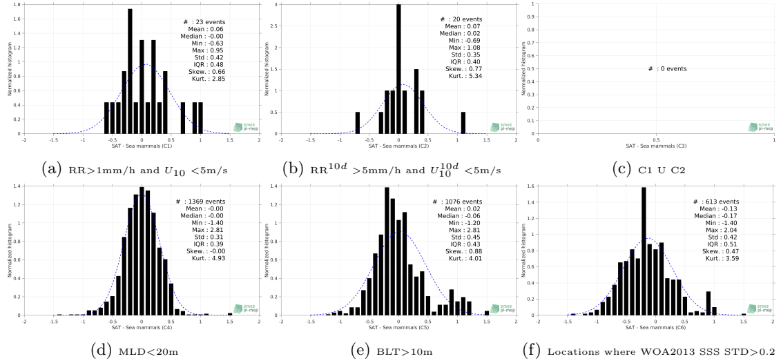
Figure 13: Normalized histogram of \Delta\text{SSS} (SMOS-L3-CATDS-CECOS-LOCEAN-V3-18DAYS-25KM - Sea mammals) for 6 different subdatasets corresponding to: \text{RR}>1\text{mm/h} and U_{10}<5\text{m/s} (a), \text{RR}^{10d}>5\text{mm/h} and U_{10}^{10d}<5\text{m/s} (b), C1 U C2 (c), \text{MLD}<20\text{m} (d), \text{BLT}>10\text{m} (e), Locations where WOA2013 SSS STD >0.2 (f).
