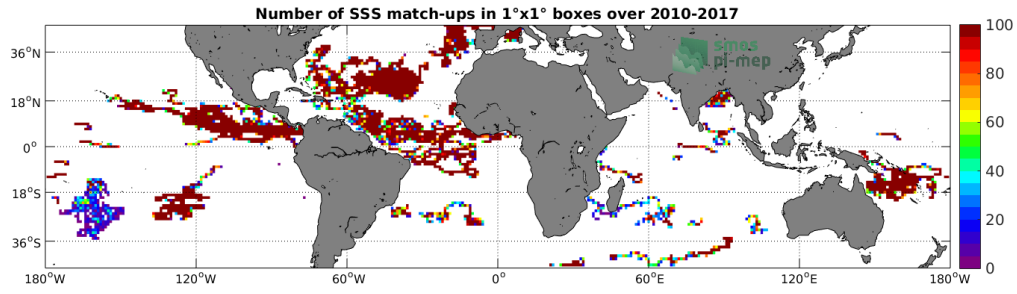
Figure 3: Number of SSS match-ups between Surface drifters SSS and the SMOS-L3-CATDS-CECOS-LOCEAN-V3-18DAYS-25KM SSS product for the Mid-Low Latitudes 45N-45S Pi-MEP region over 1°x1° boxes and for the full satellite product period.
