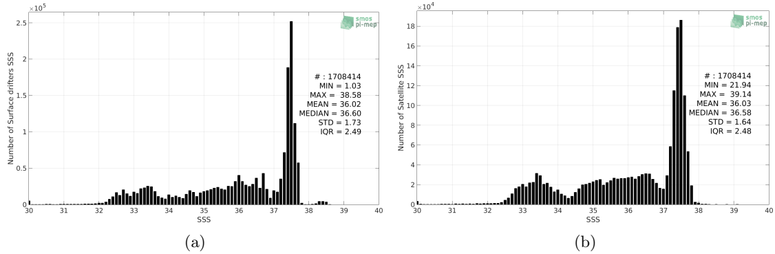
Figure 2: Histograms of SSS from Surface drifters (a) and SMOS-L3-CATDS-CECOS-LOCEAN-V3-18DAYS-25KM (b) considering all match-up pairs per bins of 0.1 over the Mid-Low Latitudes 45N-45S Pi-MEP region and for the full satellite product period.
