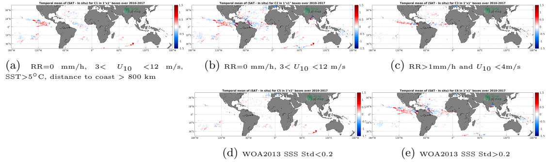
Figure 11: Temporal mean gridded over spatial boxes of size 1^\circ \times 1^\circ of \Delta SSS (SMOS-L3-CATDS-CECOS-LOCEAN-V3-18DAYS-25KM - Surface drifters) for 5 different subdatasets corresponding to: RR=0 mm/h, 3 < U_{10} < 12 m/s, SST > 5^\circ C , distance to coast > 800 km (a), RR=0 mm/h, 3 < U_{10} < 12 m/s (b), RR > 1 mm/h and U_{10} < 4 m/s (c), WOA2013 SSS Std < 0.2 (d), WOA2013 SSS Std > 0.2 (e).
