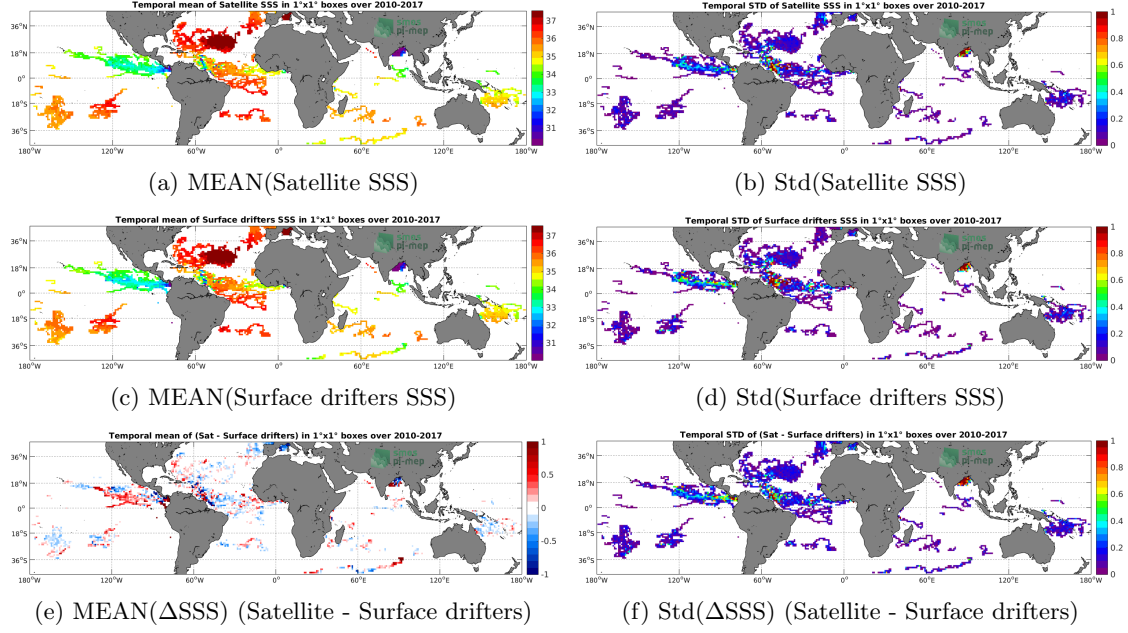
Figure 5: Temporal mean (left) and Std (right) of SSS from SMOS-L3-CATDS-CECOS-LOCEAN-V3-18DAYS-25KM (top), Surface drifters (middle), and of \Delta SSS (Satellite - Surface drifters). Only match-up pairs are used to generate these maps.
