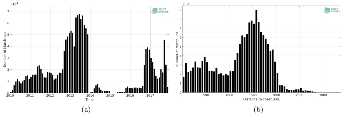
Figure 1: Number of match-ups between Surface drifters and SMOS-L3-CATDS-CECOS-LOCEAN-V3-18DAYS-25KM SSS as a function of time (a) and as function of the distance to coast (b) over the Mid-Low Latitudes 45N-45S Pi-MEP region and for the full satellite product period.
