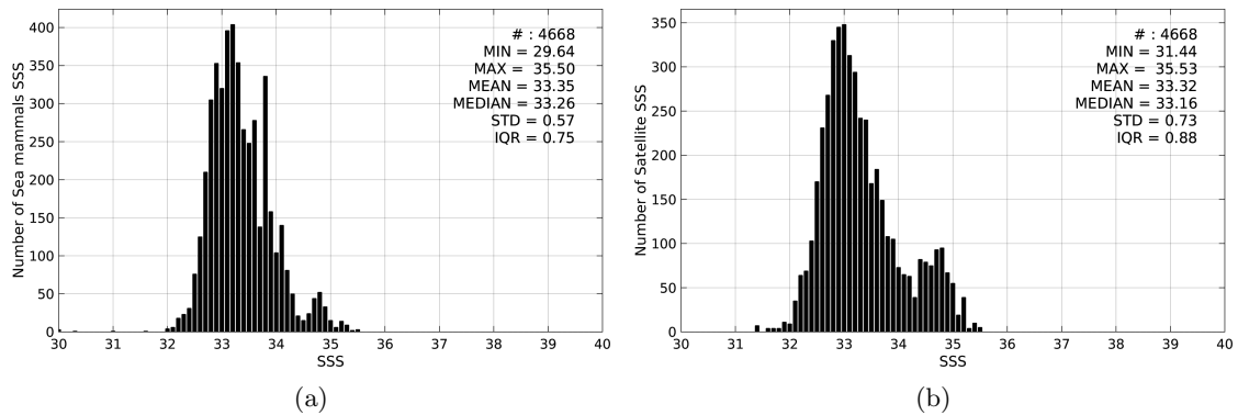
Figure 2: Histograms of SSS from Sea mammals (a) and SMOS-L3-CATDS-CECOS-LOCEAN-V2.1-9DAYS-25KM (b) considering all match-up pairs per bins of 0.1 over the Mid-Low Latitudes 45N-45S Pi-MEP region and for the full satellite product period.
