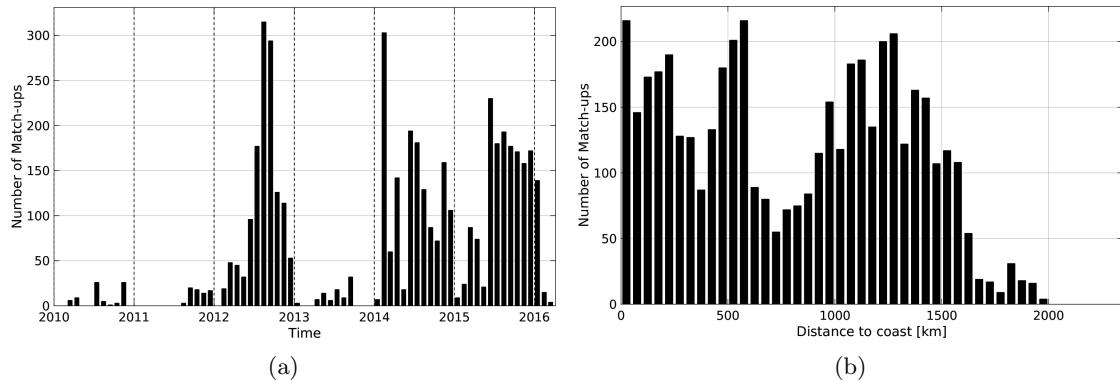
Figure 1: Number of match-ups between Sea mammals and SMOS-L3-CATDS-CECOS-LOCEAN-V2.1-9DAYS-25KM SSS as a function of time (a) and as function of the distance to coast (b) over the Mid-Low Latitudes 45N-45S Pi-MEP region and for the full satellite product period.
