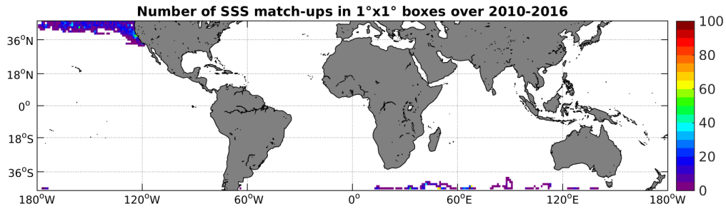
Figure 4: Number of SSS match-ups between Sea mammals SSS and the SMOS-L3-CATDS-CECOS-LOCEAN-V2.1-9DAYS-25KM SSS product for the Mid-Low Latitudes 45N-45S Pi-MEP region over 1°x1° boxes and for the full satellite product period.
