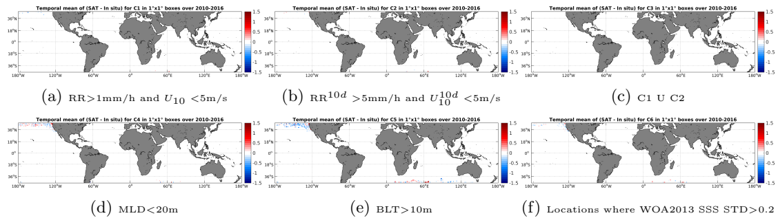
Figure 12: Temporal mean gridded over spatial boxes of size 1^\circ \times 1^\circ of \Delta SSS (SMOS-L3-CATDS-CECOS-LOCEAN-V2.1-9DAYS-25KM - Sea mammals) for 6 different subdatasets corresponding to: RR > 1 mm/h and U_{10} < 5 m/s (a), RR^{10d} > 5 mm/h and U_{10}^{10d} < 5 m/s (b), C1 U C2 (c), MLD < 20 m (d), BLT > 10 m (e), Locations where WOA2013 SSS STD > 0.2 (f).
