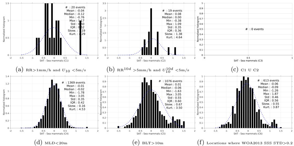
Figure 13: Normalized histogram of \Delta SSS (SMOS-L3-CATDS-CECOS-LOCEAN-V2.1-9DAYS-25KM - Sea mammals) for 6 different subdatasets corresponding to: RR > 1 mm/h and U_{10} < 5 m/s (a), RR^{10d} > 5 mm/h and U_{10}^{10d} < 5 m/s (b), C1 U C2 (c), MLD < 20 m (d), BLT > 10 m (e), Locations where WOA2013 SSS STD > 0.2 (f).
