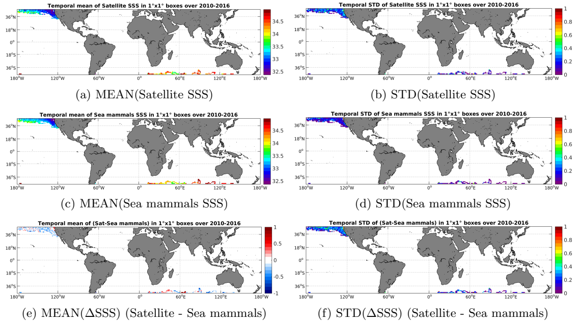
Figure 6: Temporal mean (left) and STD (right) of SSS from SMOS-L3-CATDS-CECOS-LOCEAN-V2.1-9DAYS-25KM (top), Sea mammals (middle), and of \Delta SSS (Satellite - Sea mammals). Only match-up pairs are used to generate these maps.
