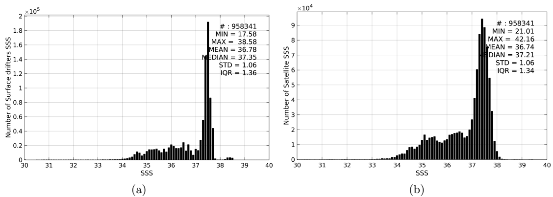
Figure 2: Histograms of SSS from Surface drifters (a) and SMOS-L3-CATDS-CECOS-LOCEAN-V2.1-9DAYS-25KM (b) considering all match-up pairs per bins of 0.1 over the Mid-Low Latitudes 45N-45S Pi-MEP region and for the full satellite product period.
