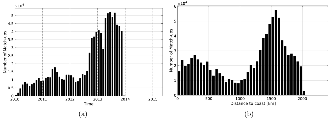
Figure 1: Number of match-ups between Surface drifters and SMOS-L3-CATDS-CECOS-LOCEAN-V2.1-9DAYS-25KM SSS as a function of time (a) and as function of the distance to coast (b) over the Mid-Low Latitudes 45N-45S Pi-MEP region and for the full satellite product period.
