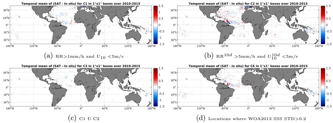
Figure 11: Temporal mean gridded over spatial boxes of size 1^\circ \times 1^\circ of \Delta SSS (SMOS-L3-CATDS-CECOS-LOCEAN-V2.1-9DAYS-25KM - Surface drifters) for 4 different subdatasets corresponding to: RR > 1\text{mm/h} and U_{10} < 5\text{m/s} (a), RR^{10d} > 5\text{mm/h} and U_{10}^{10d} < 5\text{m/s} (b), C1 U C2 (c), Locations where WOA2013 SSS STD > 0.2 (d).
