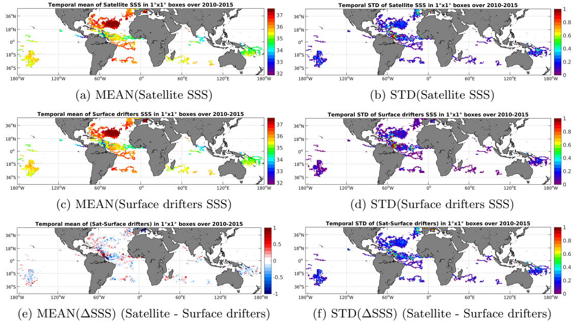
Figure 5: Temporal mean (left) and STD (right) of SSS from SMOS-L3-CATDS-CECOS-LOCEAN-V2.1-9DAYS-25KM (top), Surface drifters (middle), and of \Delta SSS (Satellite - Surface drifters). Only match-up pairs are used to generate these maps.
