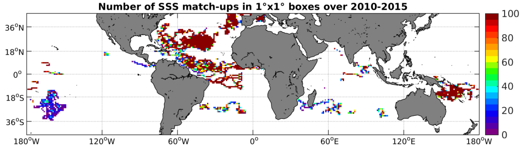
Figure 3: Number of SSS match-ups between Surface drifters SSS and the SMOS-L3-CATDS-CECOS-LOCEAN-V2.1-9DAYS-25KM SSS product for the Mid-Low Latitudes 45N-45S Pi-MEP region over 1^\circ \times 1^\circ boxes and for the full satellite product period.
