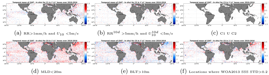
Figure 12: Temporal mean gridded over spatial boxes of size 1^\circ \times 1^\circ of \Delta SSS (SMOS-L3-CATDS-CECOS-LOCEAN-V2.1-9DAYS-25KM - Argo) for 6 different subdatasets corresponding to: RR > 1 mm/h and U_{10} < 5 m/s (a), RR^{10d} > 5 mm/h and U_{10}^{10d} < 5 m/s (b), C1 U C2 (c), MLD < 20 m (d), BLT > 10 m (e), Locations where WOA2013 SSS STD > 0.2 (f).
