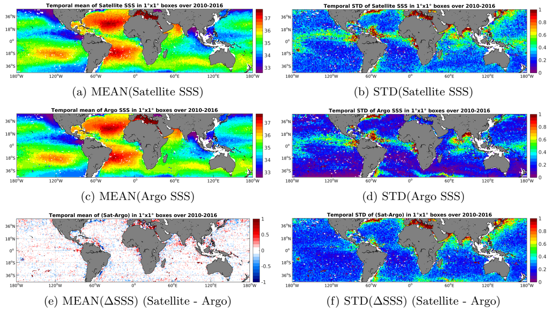
Figure 6: Temporal mean (left) and STD (right) of SSS from SMOS-L3-CATDS-CECOS-LOCEAN-V2.1-9DAYS-25KM (top), Argo (middle), and of \Delta SSS (Satellite - Argo). Only match-up pairs are used to generate these maps.
