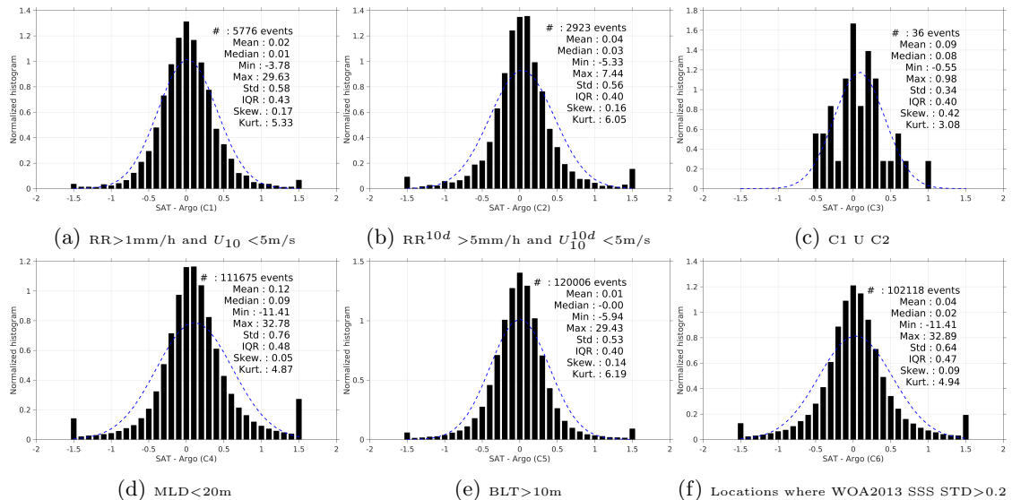
Figure 13: Normalized histogram of \Delta SSS (SMOS-L3-CATDS-CECOS-LOCEAN-V2.1-9DAYS-25KM - Argo) for 6 different subdatasets corresponding to: RR > 1 mm/h and U_{10} < 5 m/s (a), RR^{10d} > 5 mm/h and U_{10}^{10d} < 5 m/s (b), C1 U C2 (c), MLD < 20 m (d), BLT > 10 m (e), Locations where WOA2013 SSS STD > 0.2 (f).
