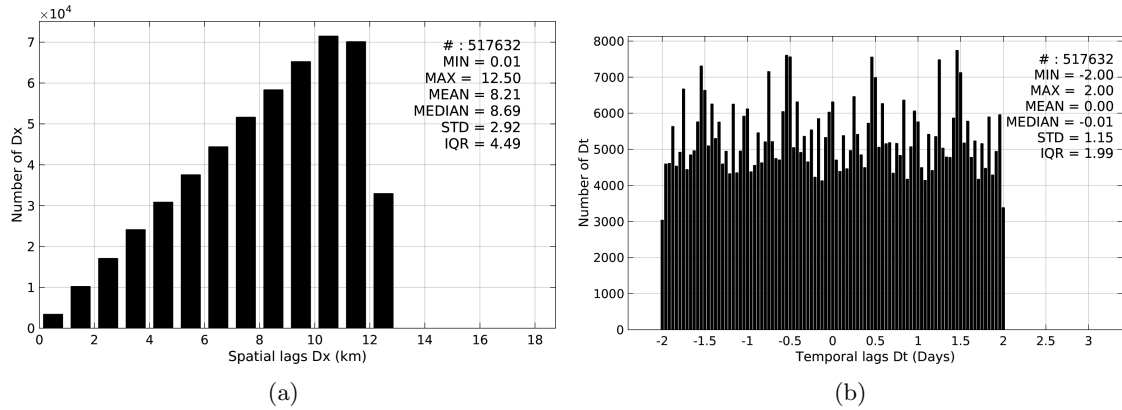
Figure 5: Histograms of the spatial (a) and temporal (b) lags between the time of the Argo measurements and the date of the corresponding SMOS-L3-CATDS-CECOS-LOCEAN-V2.1-9DAYS-25KM SSS product.
