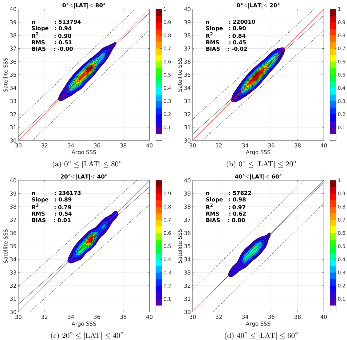
Figure 9: Contour maps of the concentration of SMOS-L3-CATDS-CECOS-LOCEAN-V2.1-9DAYS-25KM SSS (y-axis) versus Argo SSS (x-axis) at match-up pairs for different latitude bands. For each plot, the red line shows x=y . The black thin and dashed lines indicate a linear fit through the data cloud and the \pm 95\% confidence levels, respectively. The number match-up pairs n , the slope and R^2 coefficient of the linear fit, the root mean square (RMS) and the mean bias between satellite and in situ data are indicated for each latitude band in each plots.
