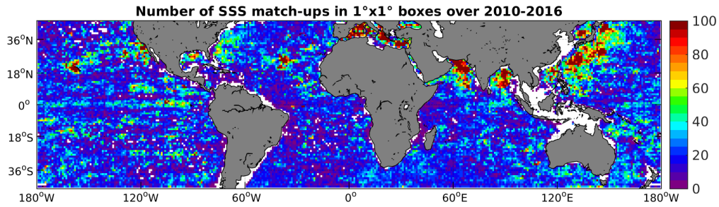
Figure 4: Number of SSS match-ups between Argo SSS and the SMOS-L3-CATDS-CECOS-LOCEAN-V2.1-9DAYS-25KM SSS product for the Mid-Low Latitudes 45N-45S Pi-MEP region over 1^\circ \times 1^\circ boxes and for the full satellite product period.
