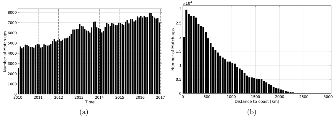
Figure 1: Number of match-ups between Argo and SMOS-L3-CATDS-CECOS-LOCEAN-V2.1-9DAYS-25KM SSS as a function of time (a) and as function of the distance to coast (b) over the Mid-Low Latitudes 45N-45S Pi-MEP region and for the full satellite product period.
