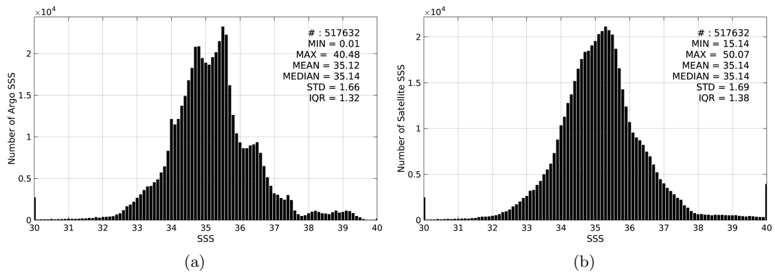
Figure 2: Histograms of SSS from Argo (a) and SMOS-L3-CATDS-CECOS-LOCEAN-V2.1-9DAYS-25KM (b) considering all match-up pairs per bins of 0.1 over the Mid-Low Latitudes 45N-45S Pi-MEP region and for the full satellite product period.
