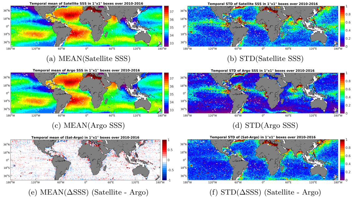
Figure 6: Temporal mean (left) and STD (right) of SSS from SMOS-L3-CATDS-CECOS-LOCEAN-V2.1-9DAYS-25KM (top), Argo (middle), and of \Delta SSS (Satellite - Argo). Only match-up pairs are used to generate these maps.
