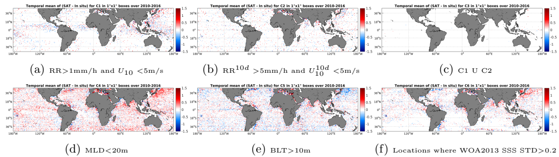
Figure 12: Temporal mean gridded over spatial boxes of size 1^\circ \times 1^\circ of \Delta SSS (SMOS-L3-CATDS-CECOS-LOCEAN-V2.1-9DAYS-25KM - Argo) for 6 different subdatasets corresponding to: RR>1mm/h and U_{10} < 5\text{m/s} (a), RR^{10d} > 5\text{mm/h} and U_{10}^{10d} < 5\text{m/s} (b), C1 U C2 (c),MLD<20m (d),BLT>10m (e),Locations where WOA2013 SSS STD>0.2 (f).
