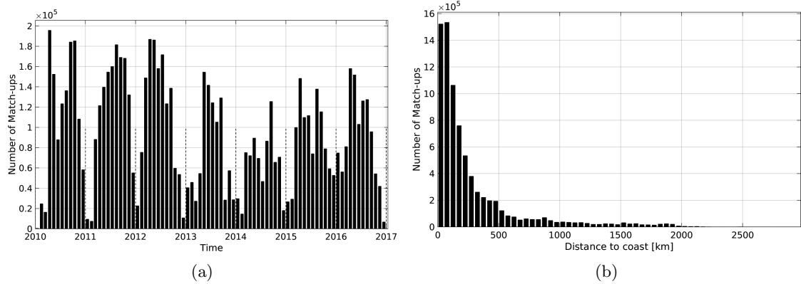
Figure 1: Number of match-ups between TSG-SAMOS and SMOS-L3-CATDS-CECOS-LOCEAN-V2-9DAYS-25KM SSS as a function of time (a) and as function of the distance to coast (b) over the Mid-Low Latitudes 45N-45S Pi-MEP region and for the full satellite product period.
