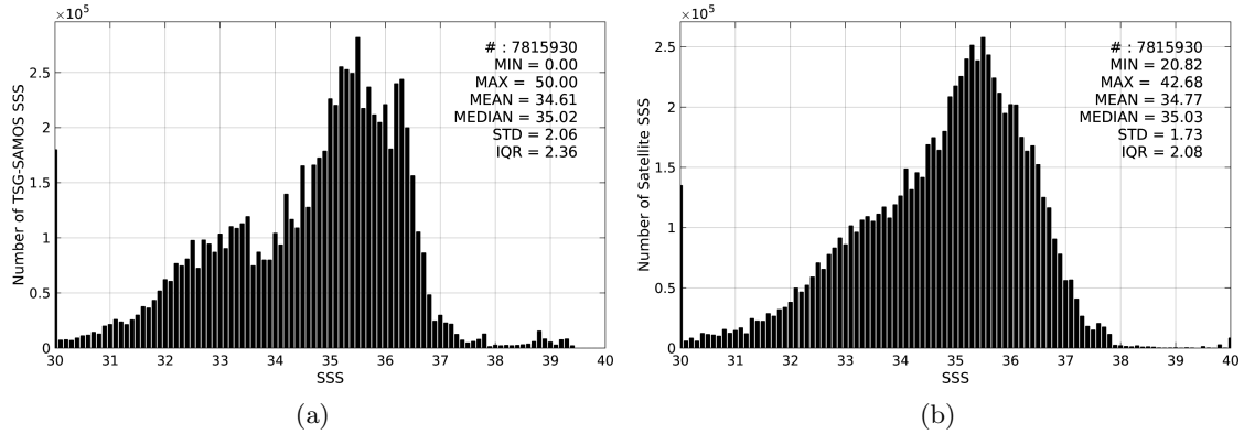
Figure 2: Histograms of SSS from TSG-SAMOS (a) and SMOS-L3-CATDS-CECOS-LOCEAN-V2-9DAYS-25KM (b) considering all match-up pairs per bins of 0.1 over the Mid-Low Latitudes 45N-45S Pi-MEP region and for the full satellite product period.
