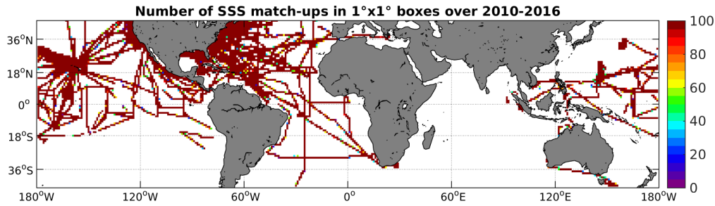
Figure 4: Number of SSS match-ups between TSG-SAMOS SSS and the SMOS-L3-CATDS-CECOS-LOCEAN-V2-9DAYS-25KM SSS product for the Mid-Low Latitudes 45N-45S Pi-MEP region over 1^\circ \times 1^\circ boxes and for the full satellite product period.
