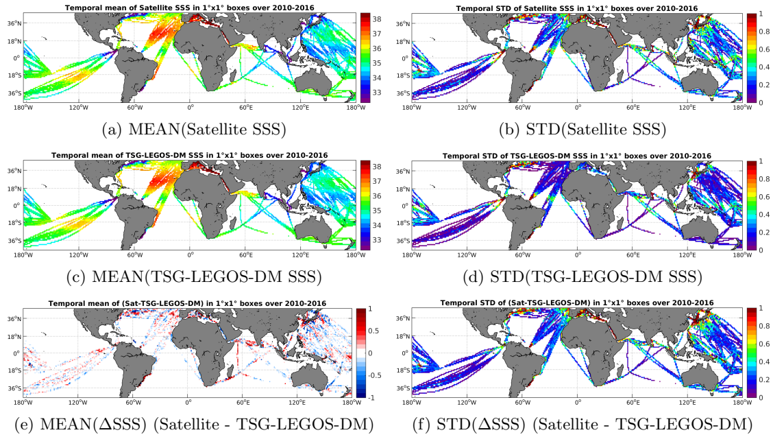
Figure 6: Temporal mean (left) and STD (right) of SSS from SMOS-L3-CATDS-CECOS-LOCEAN-V2-9DAYS-25KM (top), TSG-LEGOS-DM (middle), and of \Delta SSS (Satellite - TSG-LEGOS-DM). Only match-up pairs are used to generate these maps.
