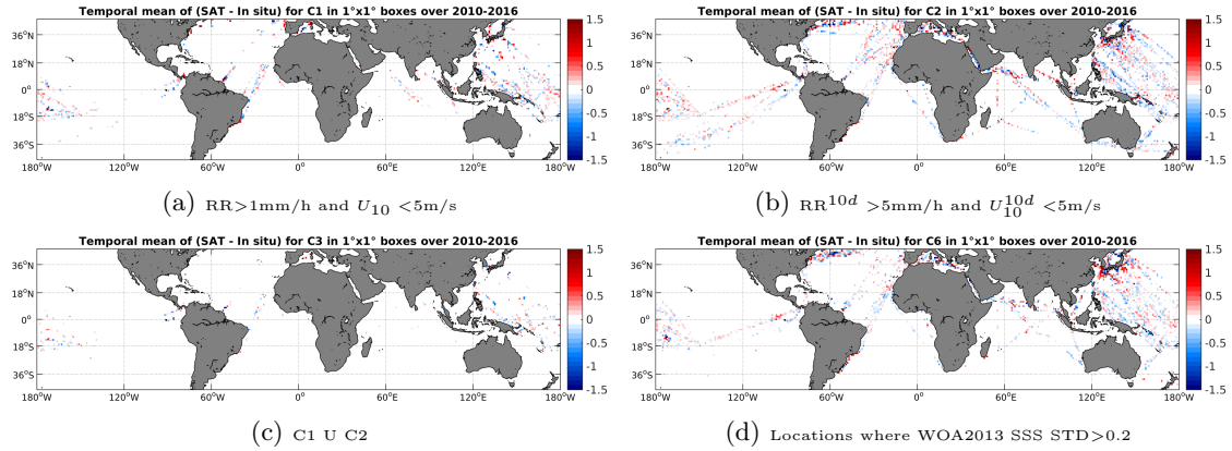
Figure 12: Temporal mean gridded over spatial boxes of size 1^\circ \times 1^\circ of \Delta SSS (SMOS-L3-CATDS-CECOS-LOCEAN-V2-9DAYS-25KM - TSG-LEGOS-DM) for 4 different subdatasets corresponding to: RR > 1\text{mm/h} and U_{10} < 5\text{m/s} (a), RR^{10d} > 5\text{mm/h} and U_{10}^{10d} < 5\text{m/s} (b), C1 U C2 (c), Locations where WOA2013 SSS STD > 0.2 (d).
