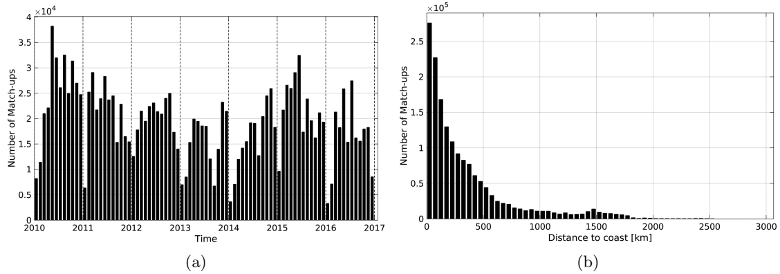
Figure 1: Number of match-ups between TSG-LEGOS-DM and SMOS-L3-CATDS-CECOS-LOCEAN-V2-9DAYS-25KM SSS as a function of time (a) and as function of the distance to coast (b) over the Mid-Low Latitudes 45N-45S Pi-MEP region and for the full satellite product period.
