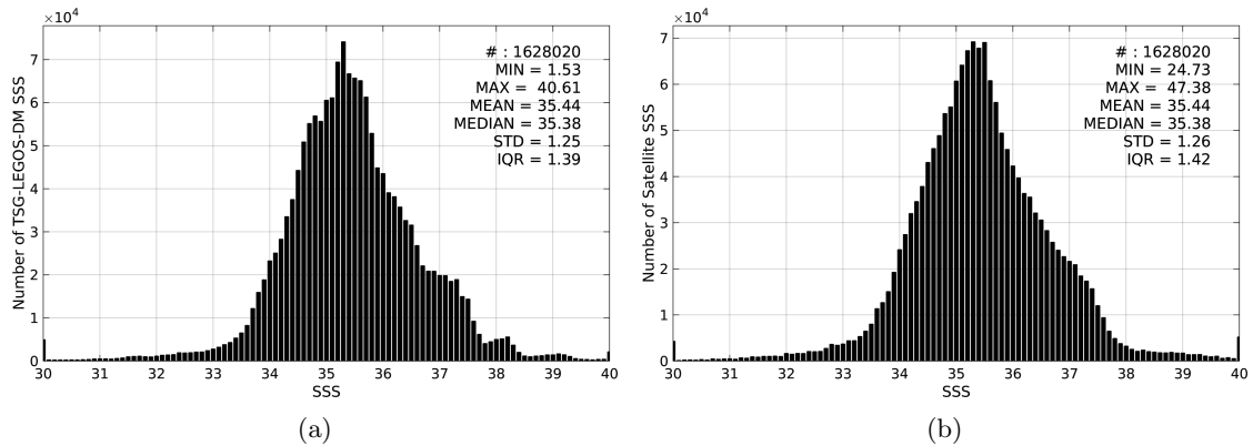
Figure 2: Histograms of SSS from TSG-LEGOS-DM (a) and SMOS-L3-CATDS-CECOS-LOCEAN-V2-9DAYS-25KM (b) considering all match-up pairs per bins of 0.1 over the Mid-Low Latitudes 45N-45S Pi-MEP region and for the full satellite product period.
