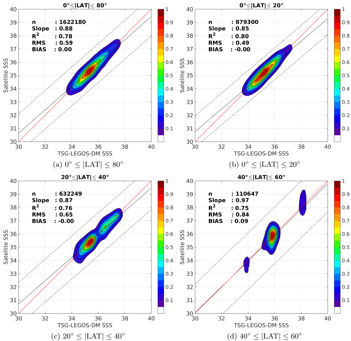
Figure 9: Contour maps of the concentration of SMOS-L3-CATDS-CECOS-LOCEAN-V2-9DAYS-25KM SSS (y-axis) versus TSG-LEGOS-DM SSS (x-axis) at match-up pairs for different latitude bands. For each plot, the red line shows x=y . The black thin and dashed lines indicate a linear fit through the data cloud and the \pm 95\% confidence levels, respectively. The number match-up pairs n , the slope and R^2 coefficient of the linear fit, the root mean square (RMS) and the mean bias between satellite and in situ data are indicated for each latitude band in each plots.
