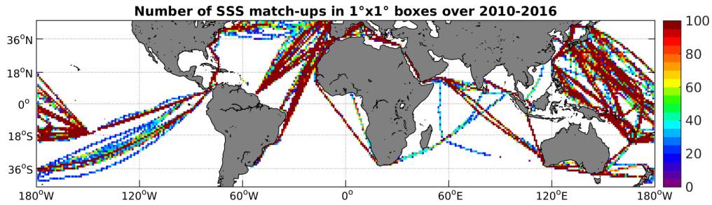
Figure 4: Number of SSS match-ups between TSG-LEGOS-DM SSS and the SMOS-L3-CATDS-CECOS-LOCEAN-V2-9DAYS-25KM SSS product for the Mid-Low Latitudes 45N-45S Pi-MEP region over 1^\circ \times 1^\circ boxes and for the full satellite product period.
