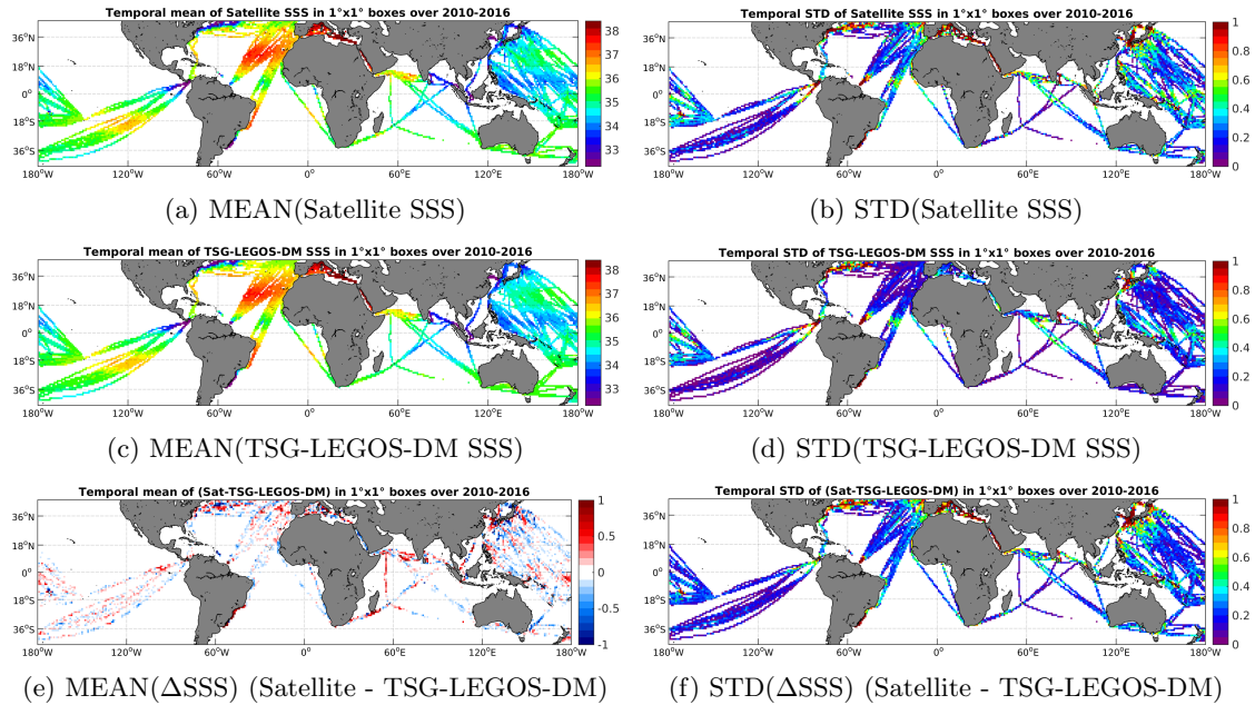
Figure 6: Temporal mean (left) and STD (right) of SSS from SMOS-L3-CATDS-CECOS-LOCEAN-V2-9DAYS-25KM (top), TSG-LEGOS-DM (middle), and of \Delta SSS (Satellite - TSG-LEGOS-DM). Only match-up pairs are used to generate these maps.
