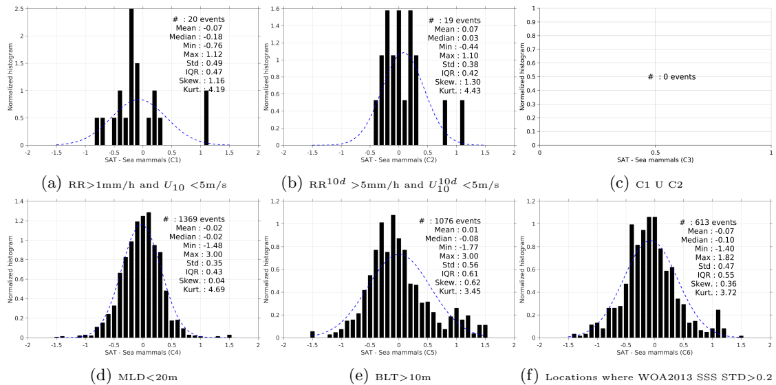
Figure 13: Normalized histogram of \Delta SSS (SMOS-L3-CATDS-CECOS-LOCEAN-V2-9DAYS-25KM - Sea mammals) for 6 different subdatasets corresponding to: RR > 1\text{mm/h} and U_{10} < 5\text{m/s} (a), RR^{10d} > 5\text{mm/h} and U_{10}^{10d} < 5\text{m/s} (b), C1 U C2 (c), MLD < 20\text{m} (d), BLT > 10\text{m} (e), Locations where WOA2013 SSS STD > 0.2 (f).
