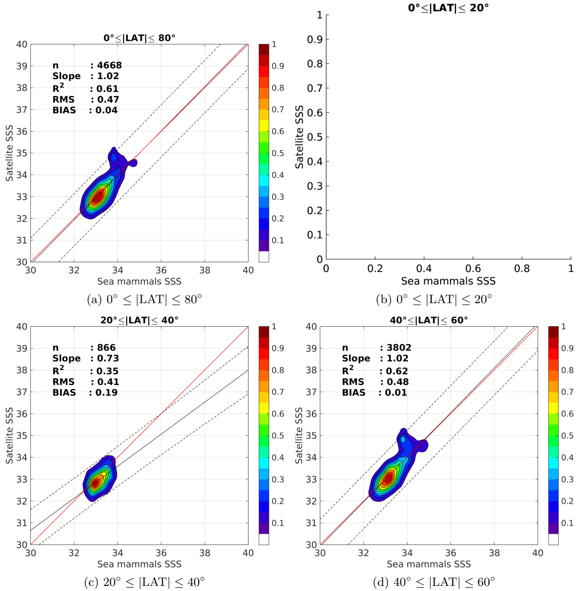
Figure 9: Contour maps of the concentration of SMOS-L3-CATDS-CECOS-LOCEAN-V2-9DAYS-25KM SSS (y-axis) versus Sea mammals SSS (x-axis) at match-up pairs for different latitude bands. For each plot, the red line shows x=y . The black thin and dashed lines indicate a linear fit through the data cloud and the \pm 95\% confidence levels, respectively. The number match-up pairs n , the slope and R^2 coefficient of the linear fit, the root mean square (RMS) and the mean bias between satellite and in situ data are indicated for each latitude band in each plots.
