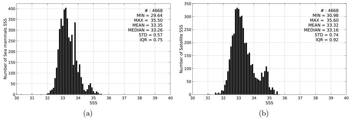
Figure 2: Histograms of SSS from Sea mammals (a) and SMOS-L3-CATDS-CECOS-LOCEAN-V2-9DAYS-25KM (b) considering all match-up pairs per bins of 0.1 over the Mid-Low Latitudes 45N-45S Pi-MEP region and for the full satellite product period.
