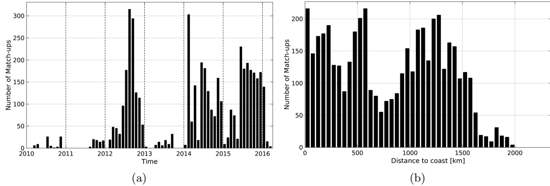
Figure 1: Number of match-ups between Sea mammals and SMOS-L3-CATDS-CECOS-LOCEAN-V2-9DAYS-25KM SSS as a function of time (a) and as function of the distance to coast (b) over the Mid-Low Latitudes 45N-45S Pi-MEP region and for the full satellite product period.
