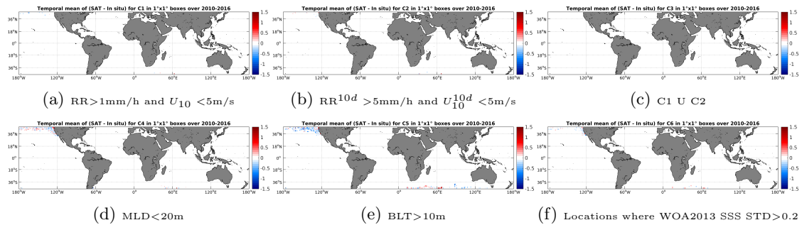
Figure 12: Temporal mean gridded over spatial boxes of size 1^\circ \times 1^\circ of \Delta SSS (SMOS-L3-CATDS-CECOS-LOCEAN-V2-9DAYS-25KM - Sea mammals) for 6 different subdatasets corresponding to: RR > 1 mm/h and U_{10} < 5 m/s (a), RR^{10d} > 5 mm/h and U_{10}^{10d} < 5 m/s (b), C1 U C2 (c), MLD < 20 m (d), BLT > 10 m (e), Locations where WOA2013 SSS STD > 0.2 (f).
