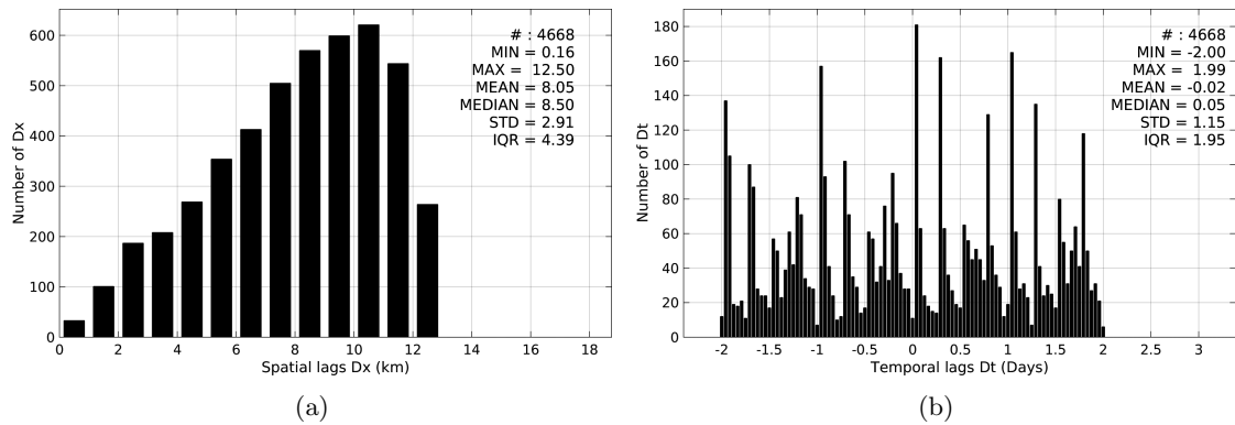
Figure 5: Histograms of the spatial (a) and temporal (b) lags between the time of the Sea mammals measurements and the date of the corresponding SMOS-L3-CATDS-CECOS-LOCEAN-V2-9DAYS-25KM SSS product.
