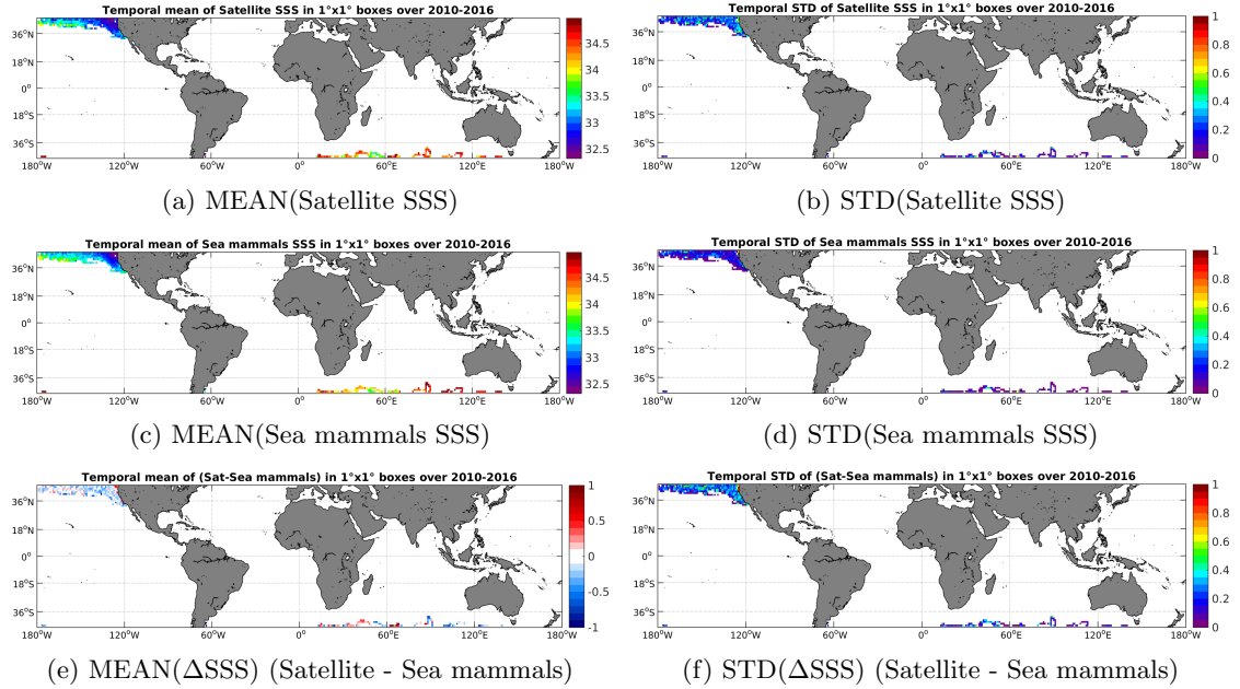
Figure 6: Temporal mean (left) and STD (right) of SSS from SMOS-L3-CATDS-CECOS-LOCEAN-V2-9DAYS-25KM (top), Sea mammals (middle), and of \Delta SSS (Satellite - Sea mammals). Only match-up pairs are used to generate these maps.
