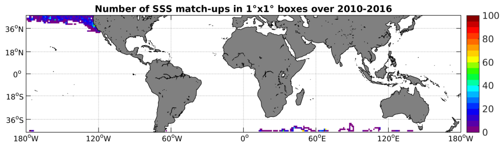
Figure 4: Number of SSS match-ups between Sea mammals SSS and the SMOS-L3-CATDS-CECOS-LOCEAN-V2-9DAYS-25KM SSS product for the Mid-Low Latitudes 45N-45S Pi-MEP region over 1^\circ \times 1^\circ boxes and for the full satellite product period.
