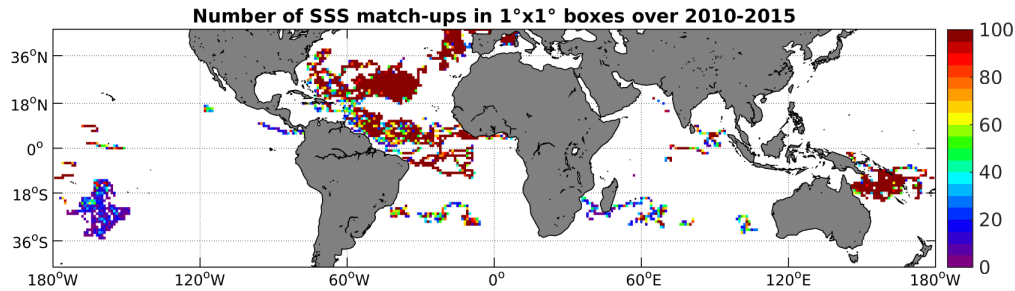
Figure 3: Number of SSS match-ups between Surface drifters SSS and the SMOS-L3-CATDS-CECOS-LOCEAN-V2-9DAYS-25KM SSS product for the Mid-Low Latitudes 45N-45S Pi-MEP region over 1^\circ \times 1^\circ boxes and for the full satellite product period.
