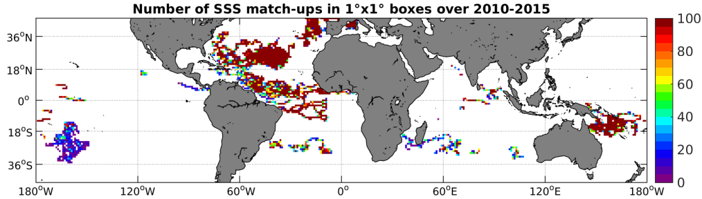
Figure 3: Number of SSS match-ups between Surface drifters SSS and the SMOS-L3-CATDS-CECOS-LOCEAN-V2-9DAYS-25KM SSS product for the Mid-Low Latitudes 45N-45S Pi-MEP region over 1°x1° boxes and for the full satellite product period.
