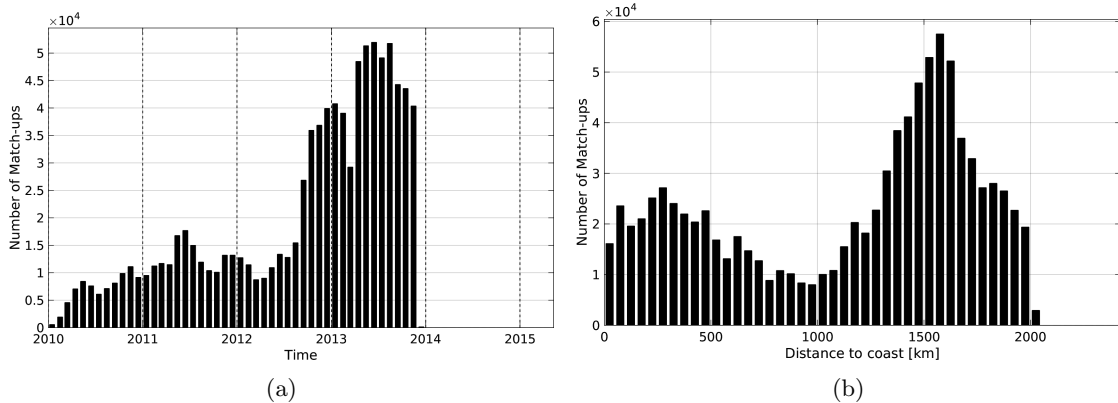
Figure 1: Number of match-ups between Surface drifters and SMOS-L3-CATDS-CECOS-LOCEAN-V2-9DAYS-25KM SSS as a function of time (a) and as function of the distance to coast (b) over the Mid-Low Latitudes 45N-45S Pi-MEP region and for the full satellite product period.
