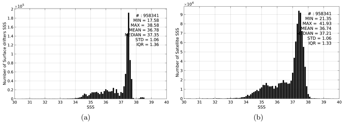
Figure 2: Histograms of SSS from Surface drifters (a) and SMOS-L3-CATDS-CECOS-LOCEAN-V2-9DAYS-25KM (b) considering all match-up pairs per bins of 0.1 over the Mid-Low Latitudes 45N-45S Pi-MEP region and for the full satellite product period.
