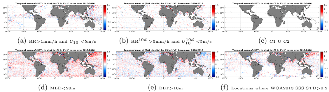
Figure 12: Temporal mean gridded over spatial boxes of size 1^\circ \times 1^\circ of \Delta SSS (SMOS-L3-CATDS-CECOS-LOCEAN-V2-9DAYS-25KM - Argo) for 6 different subdatasets corresponding to: RR > 1\text{mm/h} and U_{10} < 5\text{m/s} (a), RR^{10d} > 5\text{mm/h} and U_{10}^{10d} < 5\text{m/s} (b), C1 U C2 (c), MLD < 20\text{m} (d), BLT > 10\text{m} (e), Locations where WOA2013 SSS STD > 0.2 (f).
