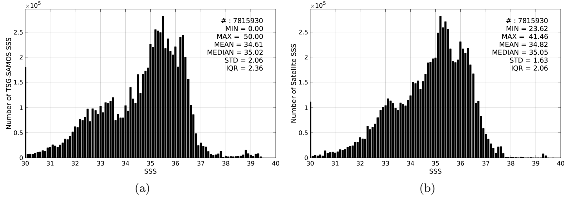
Figure 2: Histograms of SSS from TSG-SAMOS (a) and SMOS-L3-CATDS-CECOS-LOCEAN-V2-18DAYS-25KM (b) considering all match-up pairs per bins of 0.1 over the Mid-Low Latitudes 45N-45S Pi-MEP region and for the full satellite product period.
