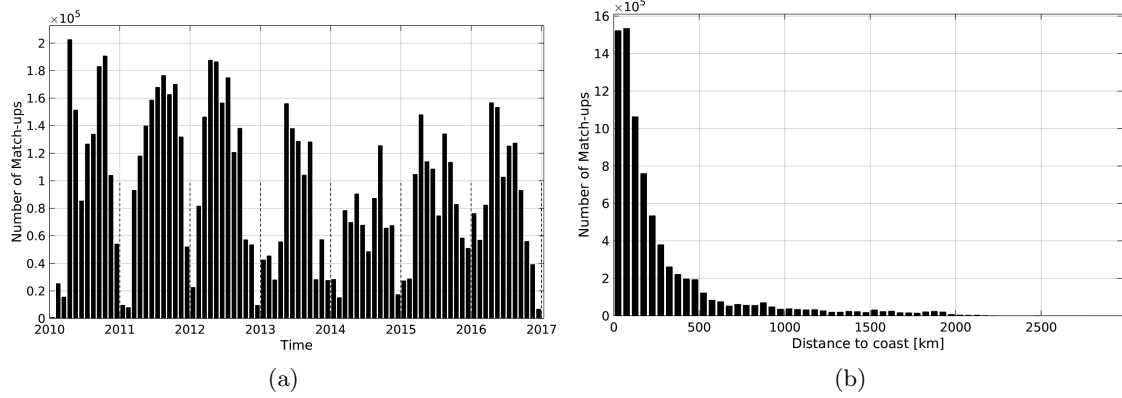
Figure 1: Number of match-ups between TSG-SAMOS and SMOS-L3-CATDS-CECOS-LOCEAN-V2-18DAYS-25KM SSS as a function of time (a) and as function of the distance to coast (b) over the Mid-Low Latitudes 45N-45S Pi-MEP region and for the full satellite product period.
