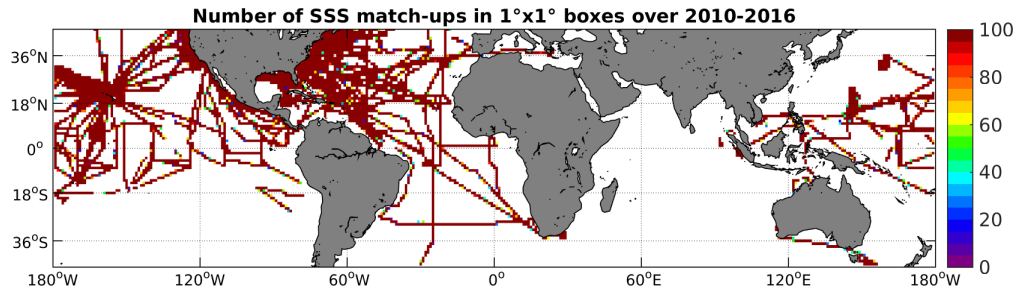
Figure 4: Number of SSS match-ups between TSG-SAMOS SSS and the SMOS-L3-CATDS-CECOS-LOCEAN-V2-18DAYS-25KM SSS product for the Mid-Low Latitudes 45N-45S Pi-MEP region over 1^\circ \times 1^\circ boxes and for the full satellite product period.
