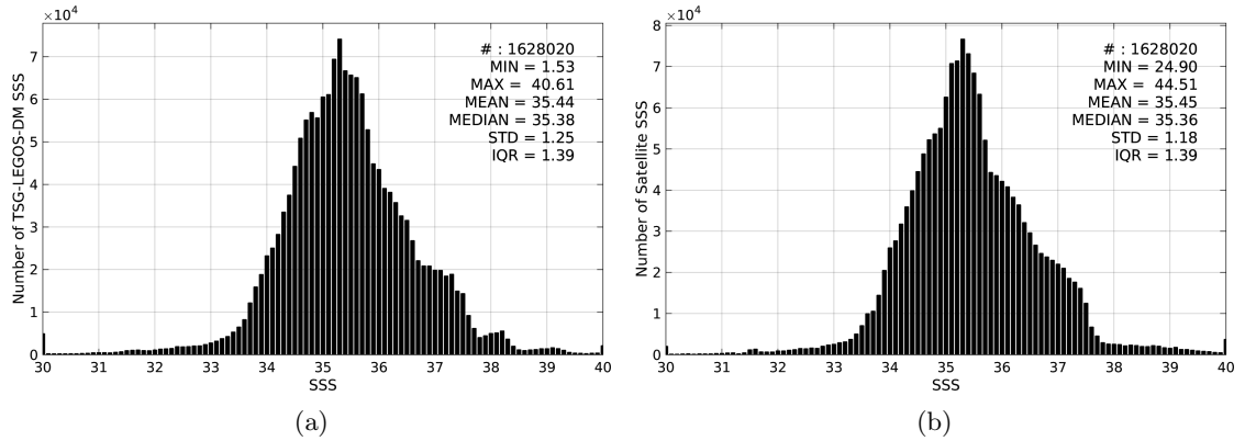
Figure 2: Histograms of SSS from TSG-LEGOS-DM (a) and SMOS-L3-CATDS-CECOS-LOCEAN-V2-18DAYS-25KM (b) considering all match-up pairs per bins of 0.1 over the Mid-Low Latitudes 45N-45S Pi-MEP region and for the full satellite product period.
