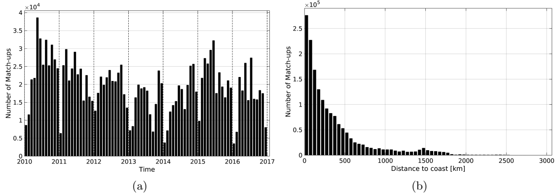
Figure 1: Number of match-ups between TSG-LEGOS-DM and SMOS-L3-CATDS-CECOS-LOCEAN-V2-18DAYS-25KM SSS as a function of time (a) and as function of the distance to coast (b) over the Mid-Low Latitudes 45N-45S Pi-MEP region and for the full satellite product period.
