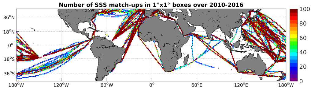
Figure 4: Number of SSS match-ups between TSG-LEGOS-DM SSS and the SMOS-L3-CATDS-CECOS-LOCEAN-V2-18DAYS-25KM SSS product for the Mid-Low Latitudes 45N-45S Pi-MEP region over 1^\circ \times 1^\circ boxes and for the full satellite product period.
