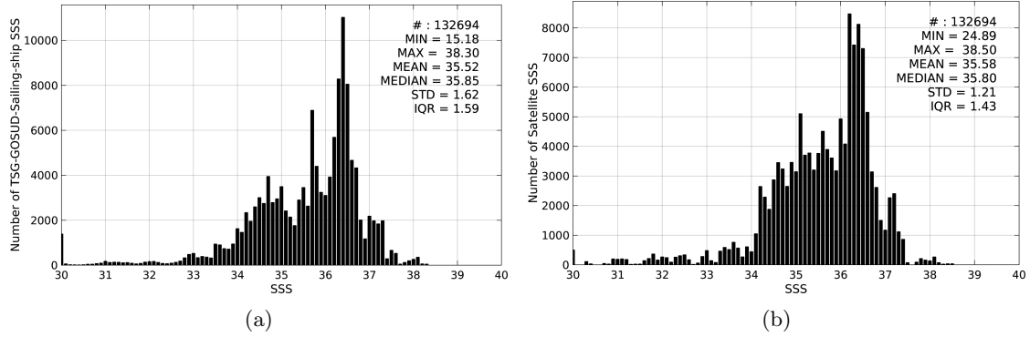
Figure 2: Histograms of SSS from TSG-GOSUD-Sailing-ship (a) and SMOS-L3-CATDS-CECOS-LOCEAN-V2-18DAYS-25KM (b) considering all match-up pairs per bins of 0.1 over the Mid-Low Latitudes 45N-45S Pi-MEP region and for the full satellite product period.
