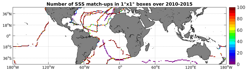
Figure 4: Number of SSS match-ups between TSG-GOSUD-Sailing-ship SSS and the SMOS-L3-CATDS-CECOS-LOCEAN-V2-18DAYS-25KM SSS product for the Mid-Low Latitudes 45N-45S Pi-MEP region over 1°x1° boxes and for the full satellite product period.
