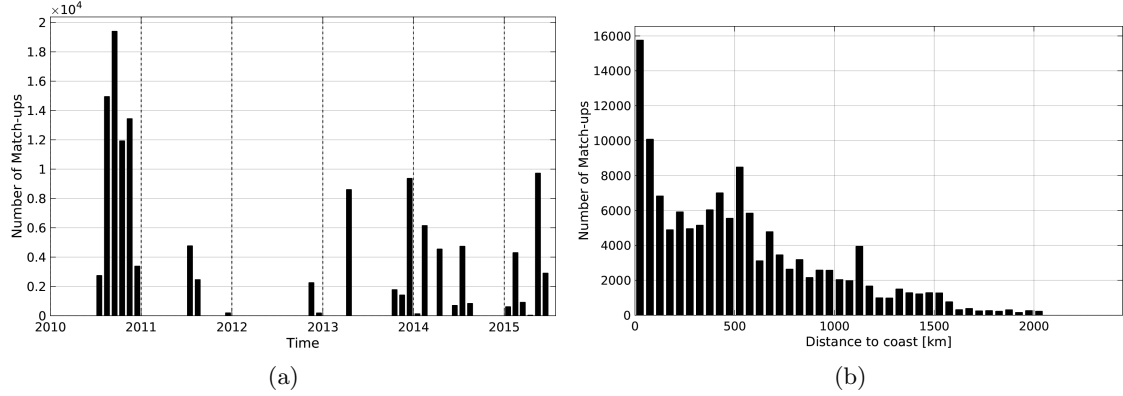
Figure 1: Number of match-ups between TSG-GOSUD-Sailing-ship and SMOS-L3-CATDS-CECOS-LOCEAN-V2-18DAYS-25KM SSS as a function of time (a) and as function of the distance to coast (b) over the Mid-Low Latitudes 45N-45S Pi-MEP region and for the full satellite product period.
