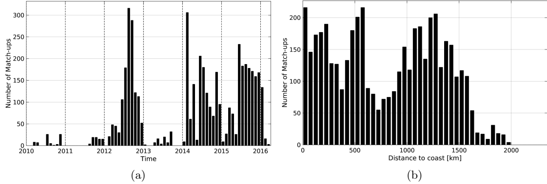
Figure 1: Number of match-ups between Sea mammals and SMOS-L3-CATDS-CECOS-LOCEAN-V2-18DAYS-25KM SSS as a function of time (a) and as function of the distance to coast (b) over the Mid-Low Latitudes 45N-45S Pi-MEP region and for the full satellite product period.
