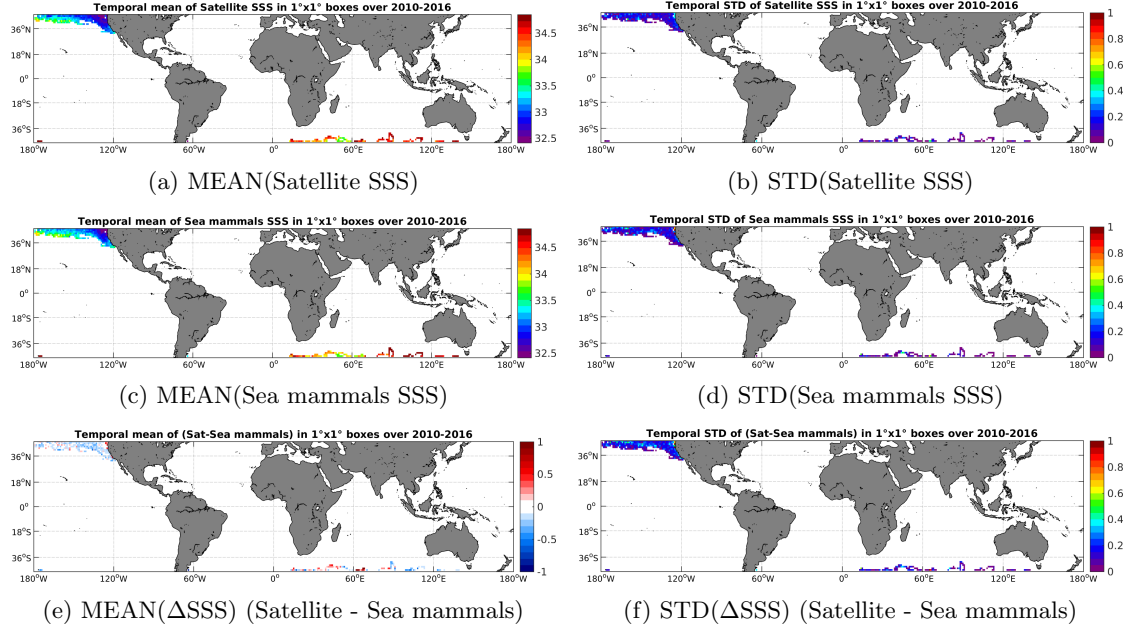
Figure 6: Temporal mean (left) and STD (right) of SSS from SMOS-L3-CATDS-CECOS-LOCEAN-V2-18DAYS-25KM (top), Sea mammals (middle), and of \Delta SSS (Satellite - Sea mammals). Only match-up pairs are used to generate these maps.
