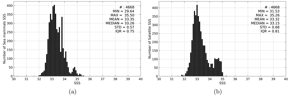
Figure 2: Histograms of SSS from Sea mammals (a) and SMOS-L3-CATDS-CECOS-LOCEAN-V2-18DAYS-25KM (b) considering all match-up pairs per bins of 0.1 over the Mid-Low Latitudes 45N-45S Pi-MEP region and for the full satellite product period.
