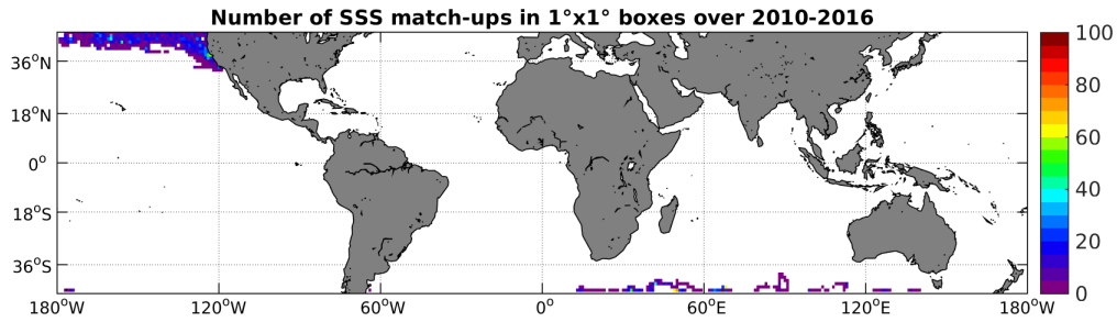
Figure 4: Number of SSS match-ups between Sea mammals SSS and the SMOS-L3-CATDS-CECOS-LOCEAN-V2-18DAYS-25KM SSS product for the Mid-Low Latitudes 45N-45S Pi-MEP region over 1^\circ \times 1^\circ boxes and for the full satellite product period.
