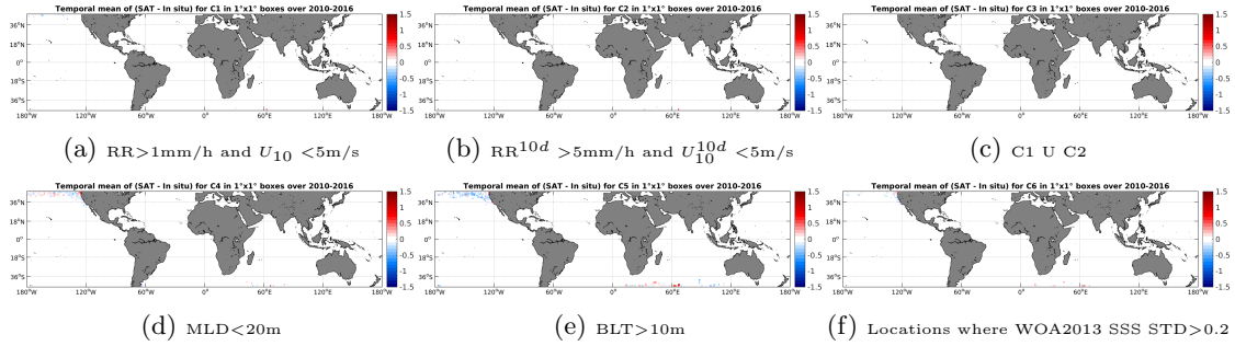
Figure 12: Temporal mean gridded over spatial boxes of size 1^\circ \times 1^\circ of \Delta SSS (SMOS-L3-CATDS-CECOS-LOCEAN-V2-18DAYS-25KM - Sea mammals) for 6 different subdatasets corresponding to: RR > 1\text{mm/h} and U_{10} < 5\text{m/s} (a), RR^{10d} > 5\text{mm/h} and U_{10}^{10d} < 5\text{m/s} (b), C1 U C2 (c), MLD < 20\text{m} (d), BLT > 10\text{m} (e), Locations where WOA2013 SSS STD > 0.2 (f).
